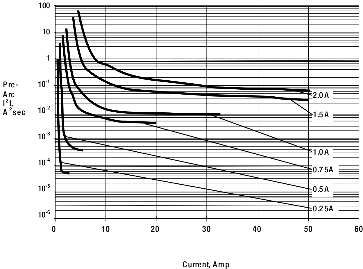
FUSE PRE-ARC JOULE INTEGRALS VS CURRENT FOR TYPE F0402E (TYPICAL)
