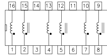
F-1504 & F-1508 6 Line 16-Pin Schematic
