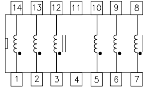
F-1500 6 Line 14-Pin Schematic
