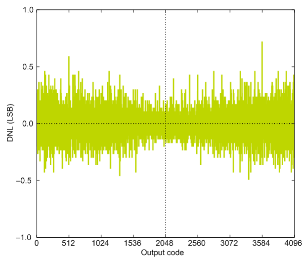
5VDIFF Reference
