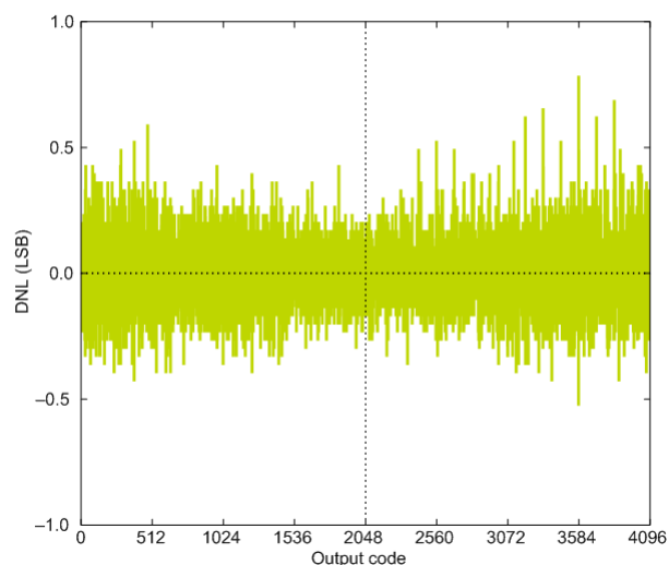
2.5 V Reference
