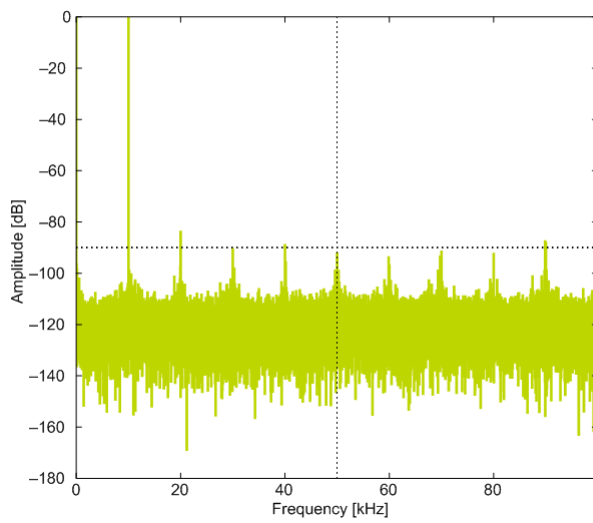
2XVDDVSS Reference
