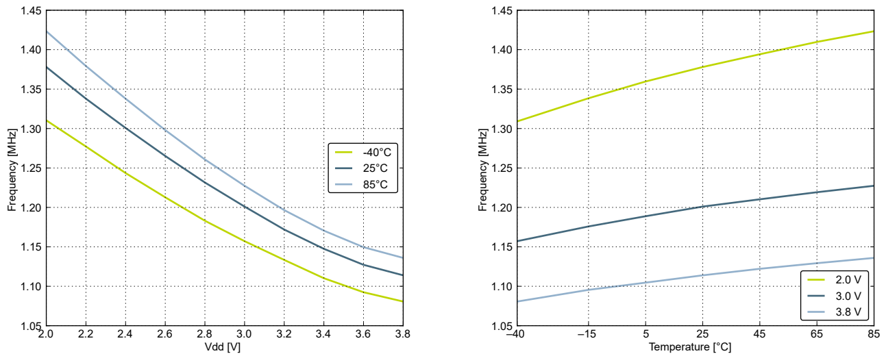
Figure 4.8. Calibrated HFRCO 1 MHz Band Frequency vs Supply Voltage and Temperature
