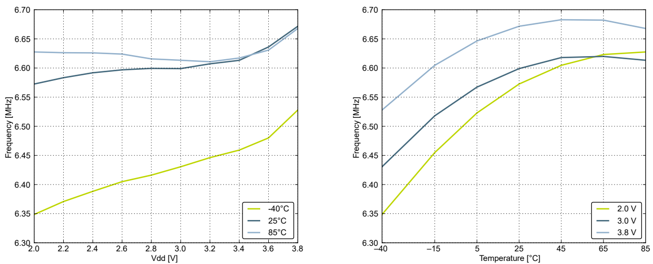
Figure 4.9. Calibrated HFRCO 7 MHz Band Frequency vs Supply Voltage and Temperature
