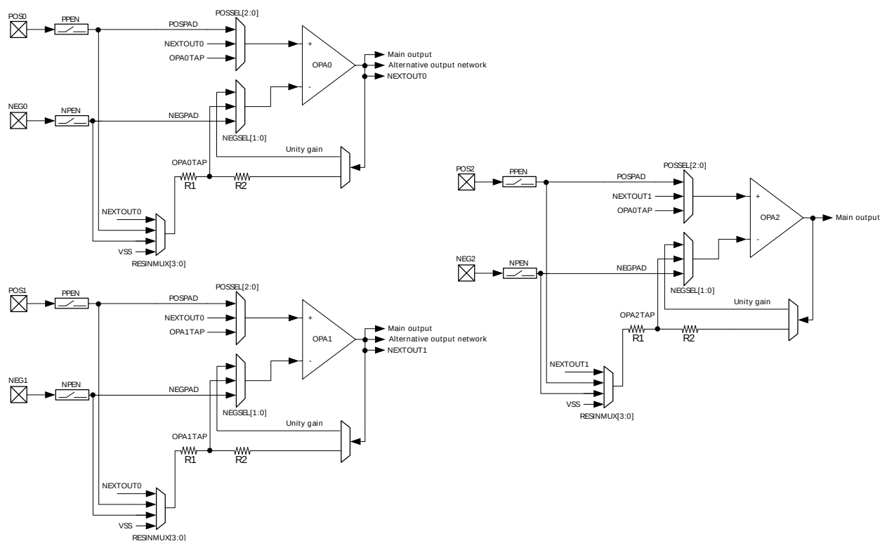
Figure 30.2. OPAMP Overview
