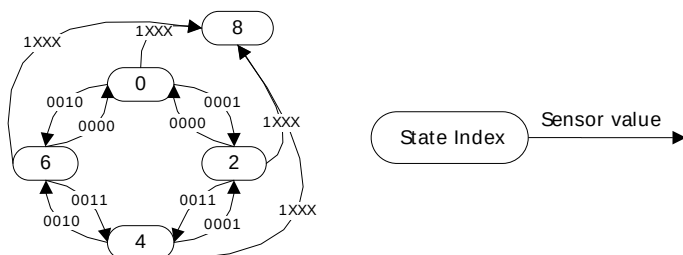
Figure 25.14. FSM example 2
