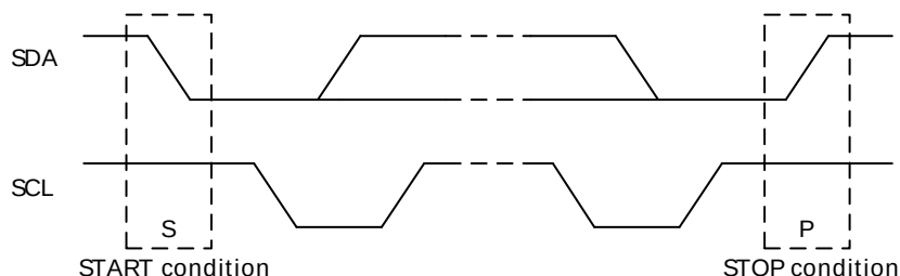
Figure 16.3. I 2 C START and STOP Conditions
