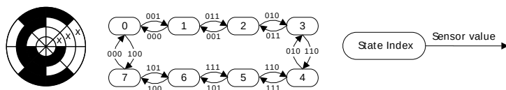
Figure 25.13. FSM example 1
