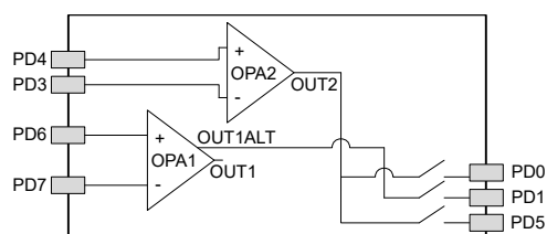
Figure 5.2. Opamp Pinout
