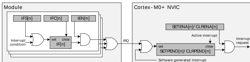
Figure 5.1. Interrupt Operation
