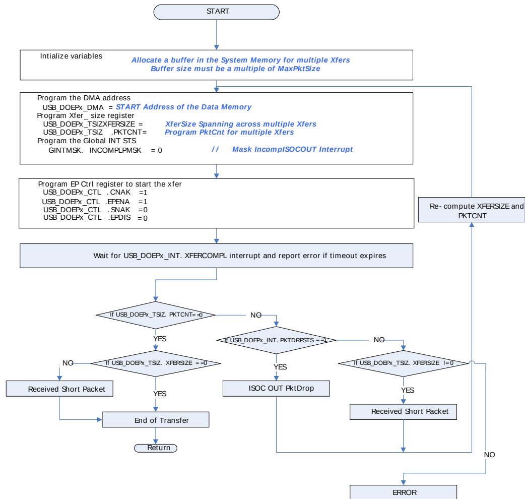
Note: 1. The (micro) frame number and PID field are not updated for Periodic OUT packets 2. In Periodic OUT transfers any short packet results in an XferComplete interrupt and disables the endpoint. The application must reenoble the endpoint with recalculated values of XferSize and PktCnt 3. The application must reenoble the endpoint after dropped packets for ISOC OUT
