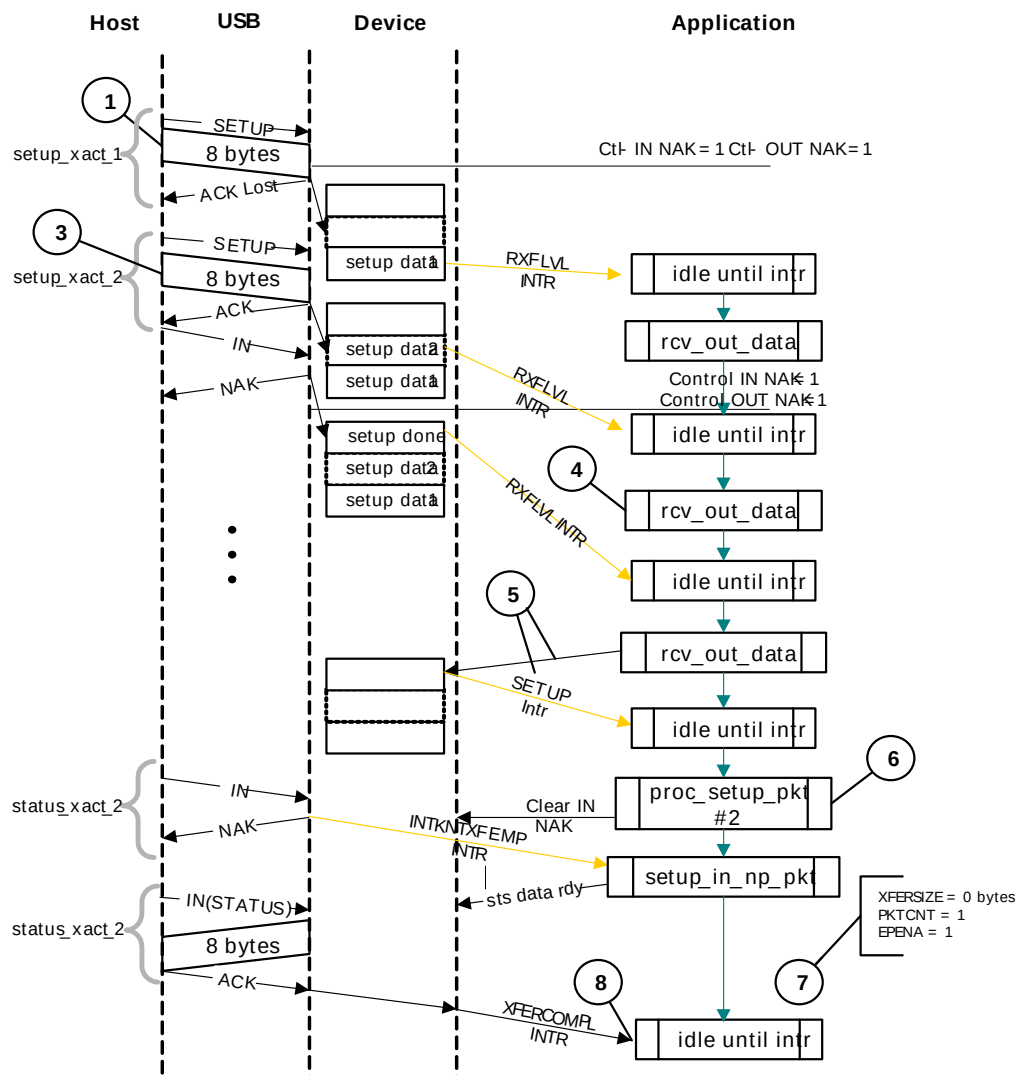
Figure 15.17. Two-Stage Control Transfer
