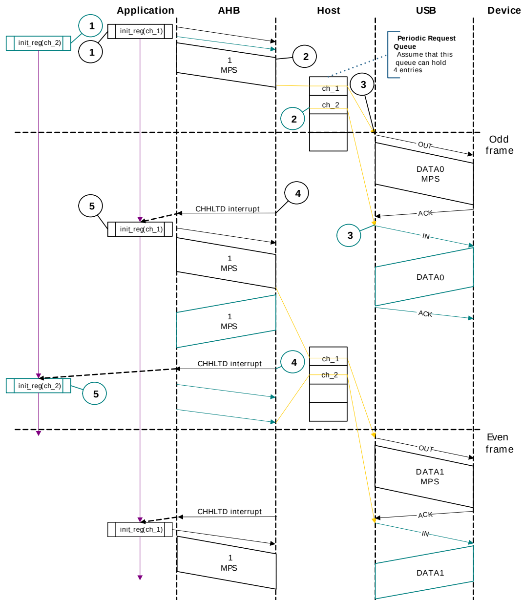
Figure 15.13. Normal Interrupt OUT/IN Transactions in DMA Mode
