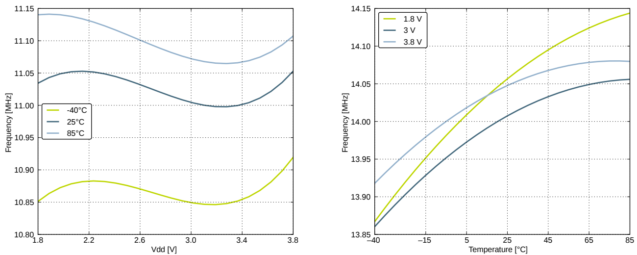
Figure 4.24. Calibrated HFRCO 14 MHz Band Frequency vs Supply Voltage and Temperature
