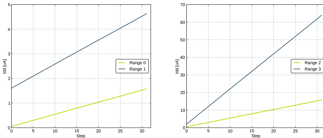
Figure 4.37. IDAC Linearity
