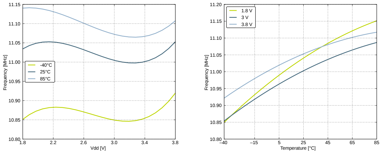
Figure 4.23. Calibrated HFRCO 11 MHz Band Frequency vs Supply Voltage and Temperature
