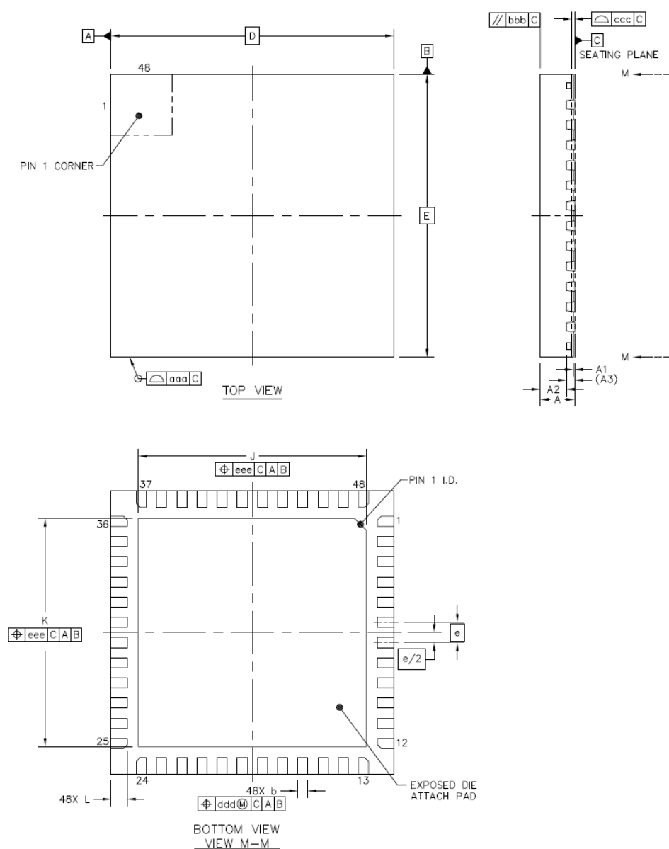
Figure 5.2. QFN48
