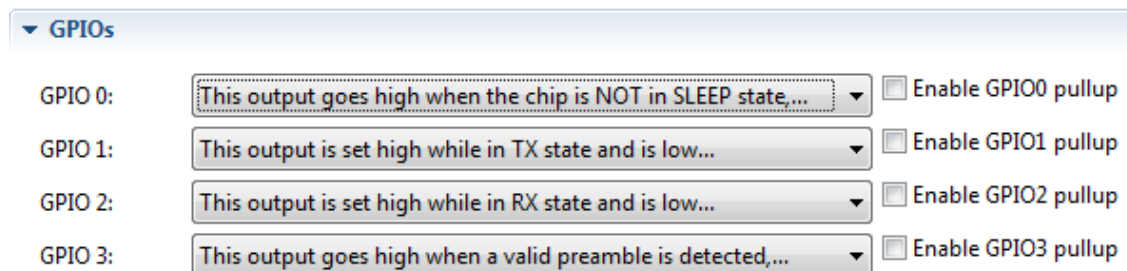
Figure 6.5. GPIO Configuration for Power Optimization
