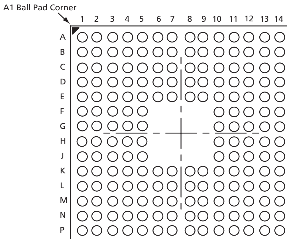
Figure 2-5 • 180-Pin CSP
