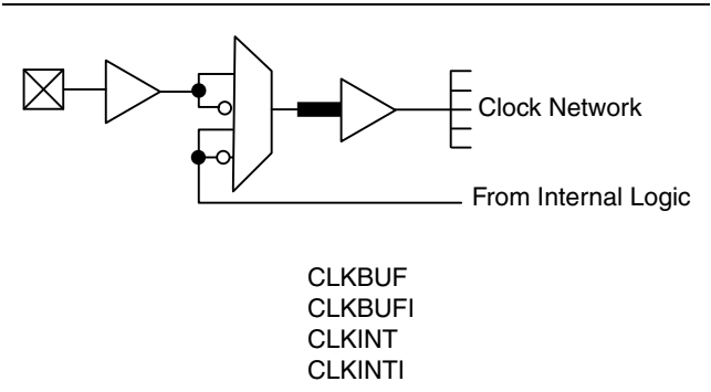
Figure 6 • eX Routed Clock Buffer
