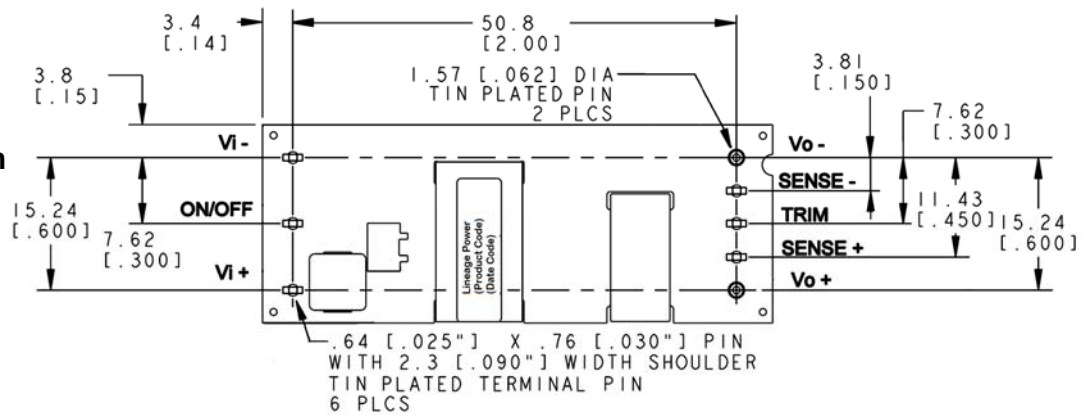
Bottom View
