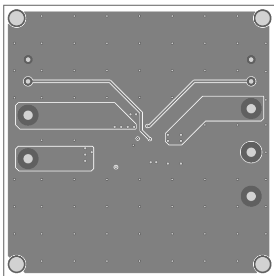
Figure 3: Inner2 Layer
