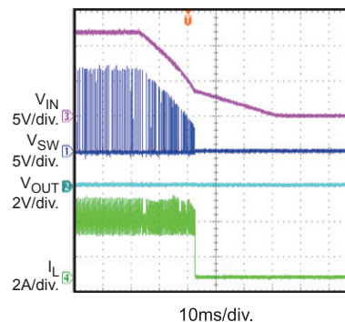
LED+ Short to GND Input Power Off
