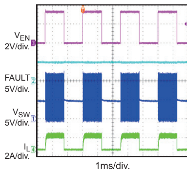
PWM Dimming
