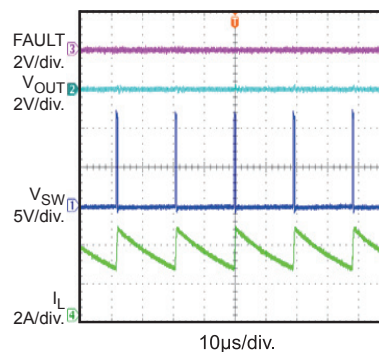
LED+ Short to GND
