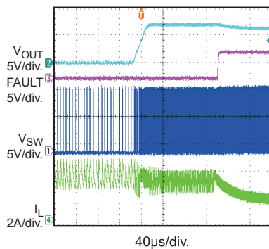
LED+ Short to GND Recovery
