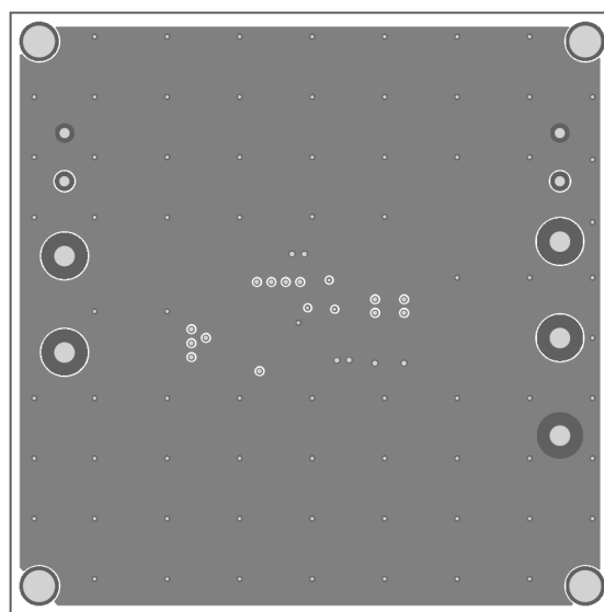
Figure 2: Inner1 Layer
