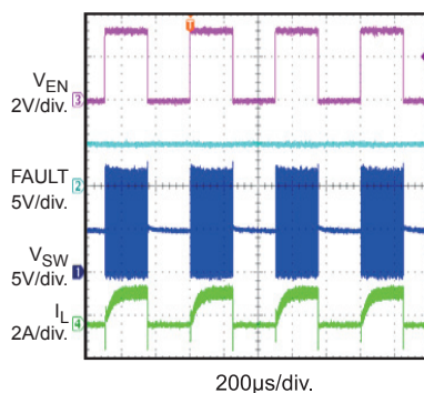
PWM Dimming
