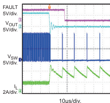
LED+ Short to GND Entry
