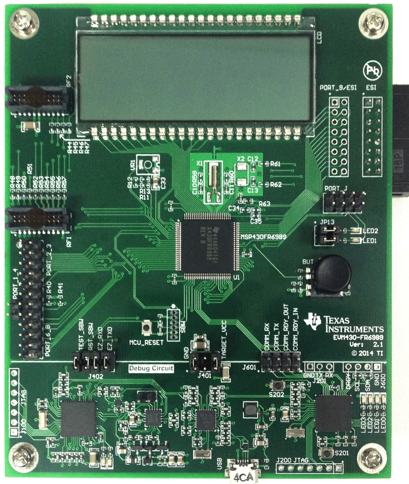
Figure 2. Main Board
