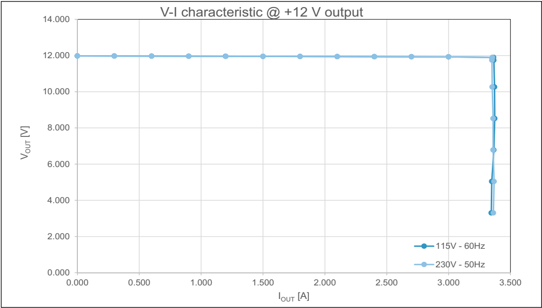
Figure 2. CV-CC regulation @ 12Vout
