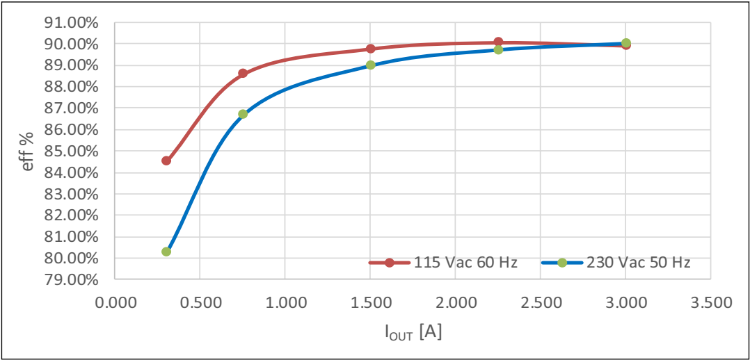
Figure 6. Efficiency plot @ 9 V output
