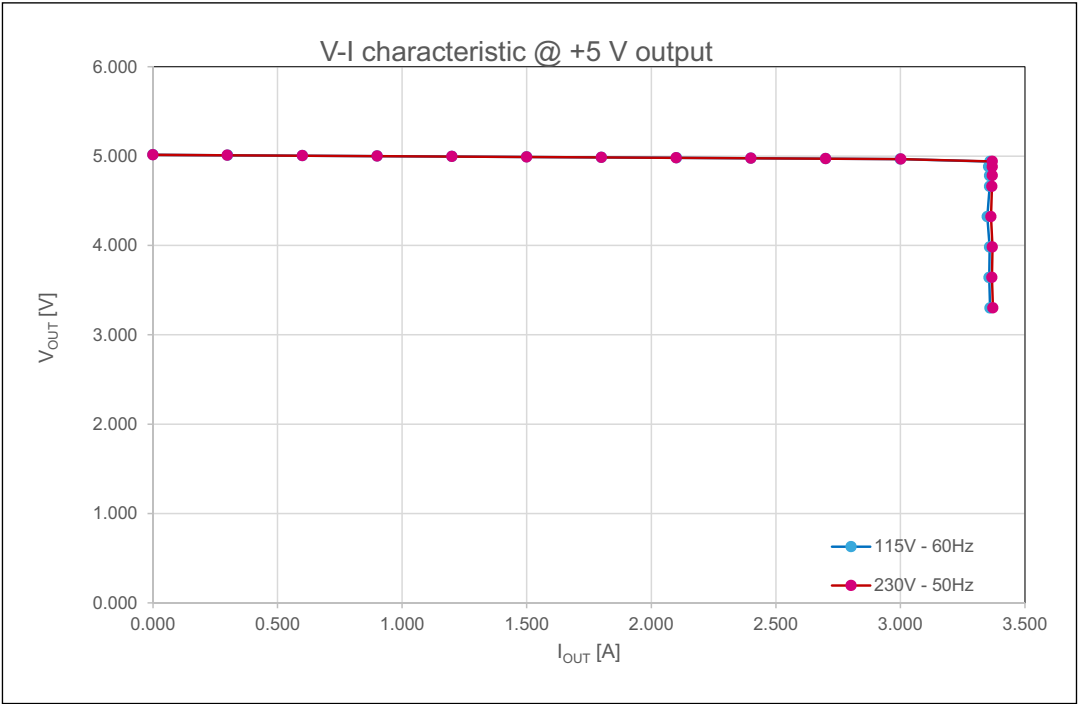
Figure 4. CV-CC regulation @ 5Vout
