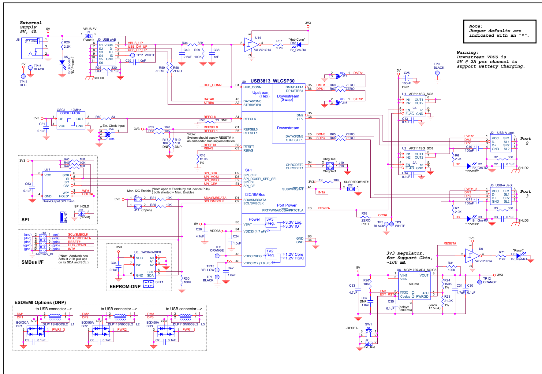
FIGURE B-1: EVB-USB3813 EVALUATION BOARD SCHEMATIC
