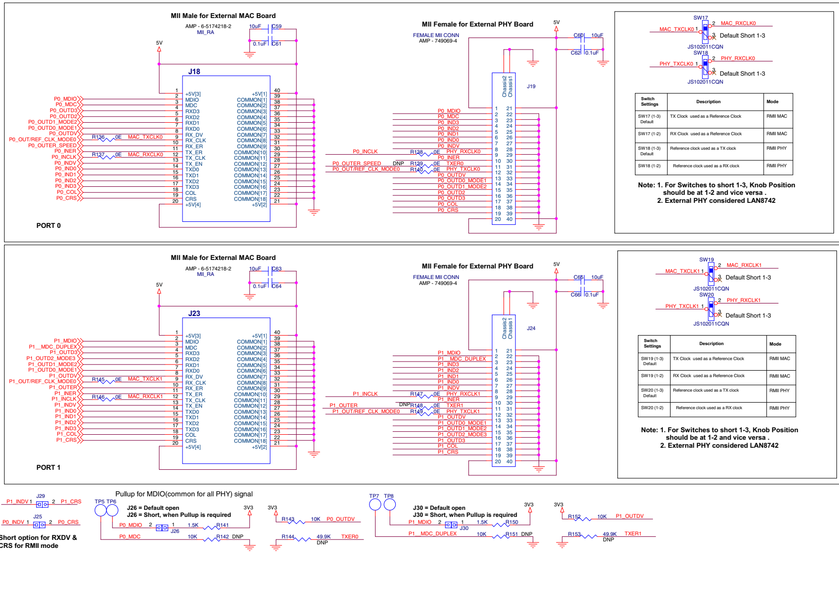
FIGURE B-8: EVB-LAN9355 EVALUATION BOARD SCHEMATIC 8
