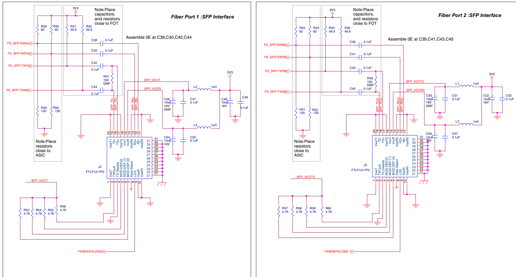
FIGURE B-5: EVB-LAN9355 EVALUATION BOARD SCHEMATIC 5
