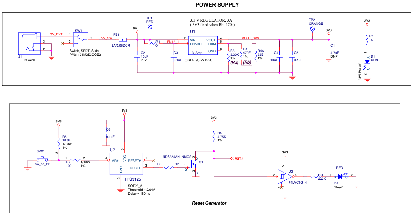
FIGURE B-2: EVB-LAN9355 EVALUATION BOARD SCHEMATIC 2
