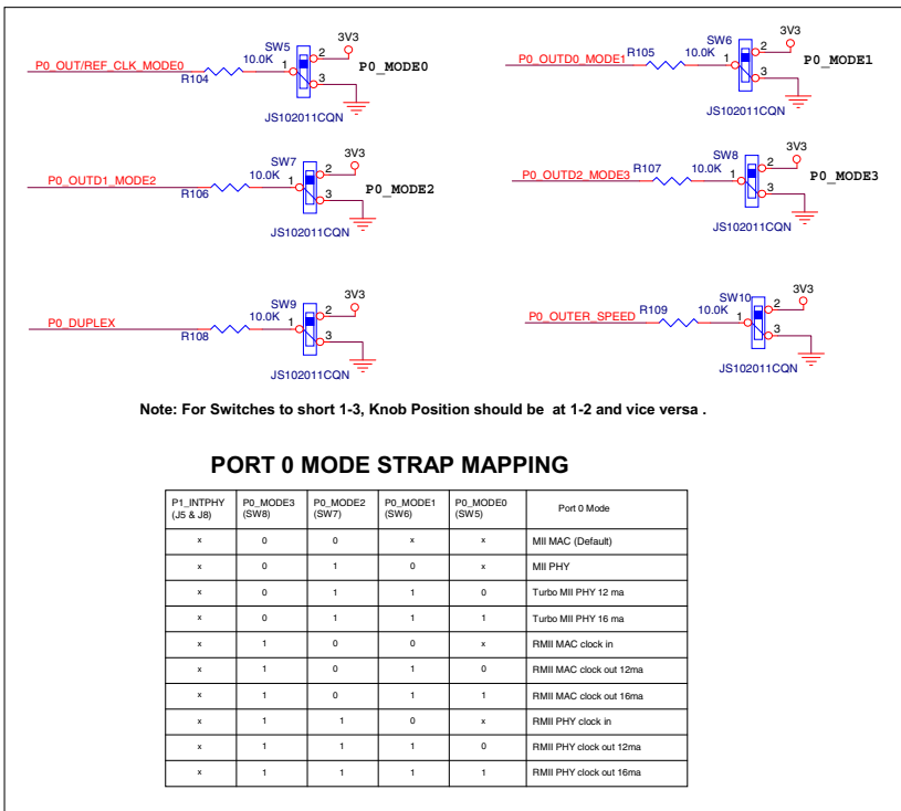
FIGURE B-7: EVB-LAN9355 EVALUATION BOARD SCHEMATIC 7
