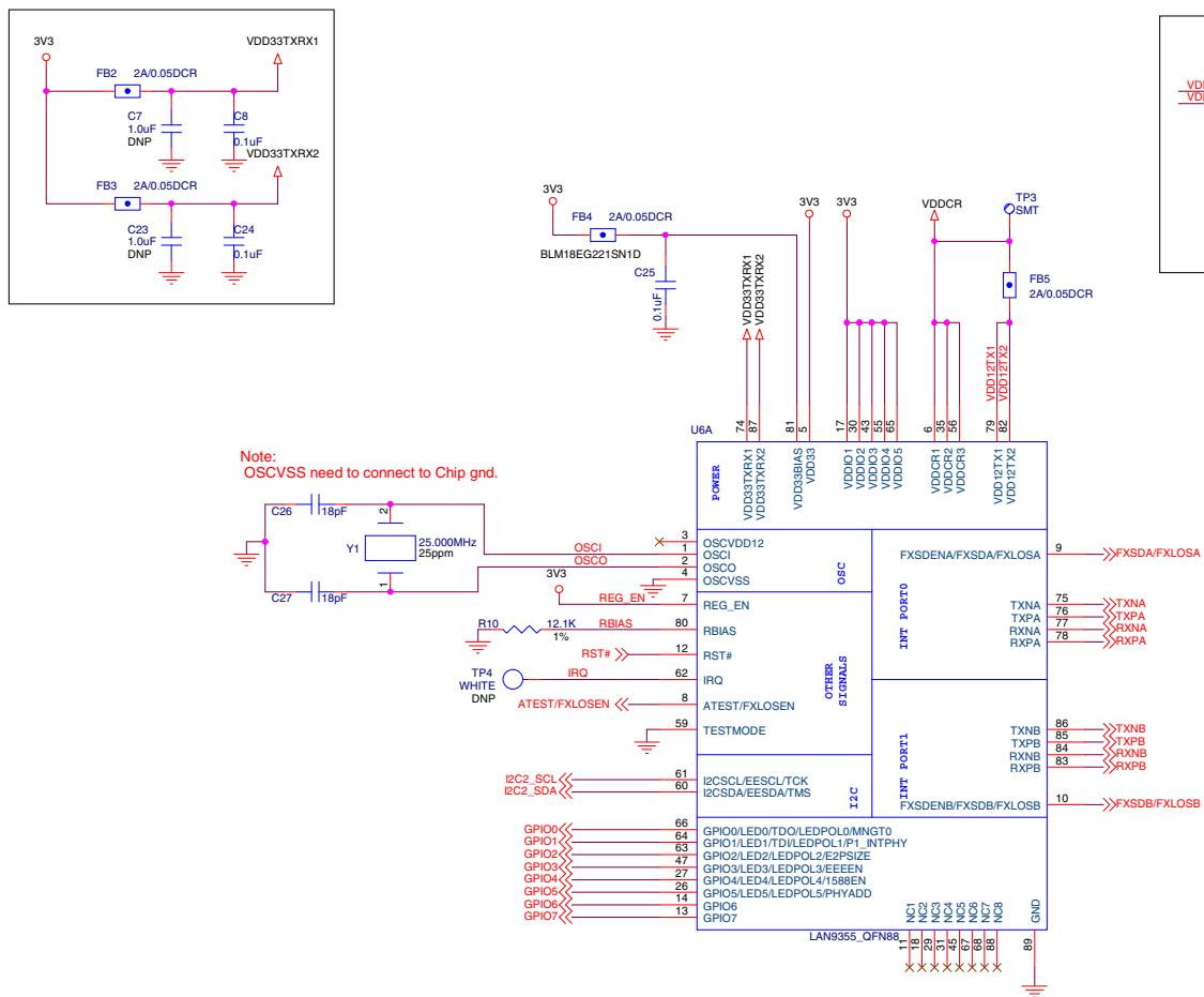
FIGURE B-3: EVB-LAN9355 EVALUATION BOARD SCHEMATIC 3
