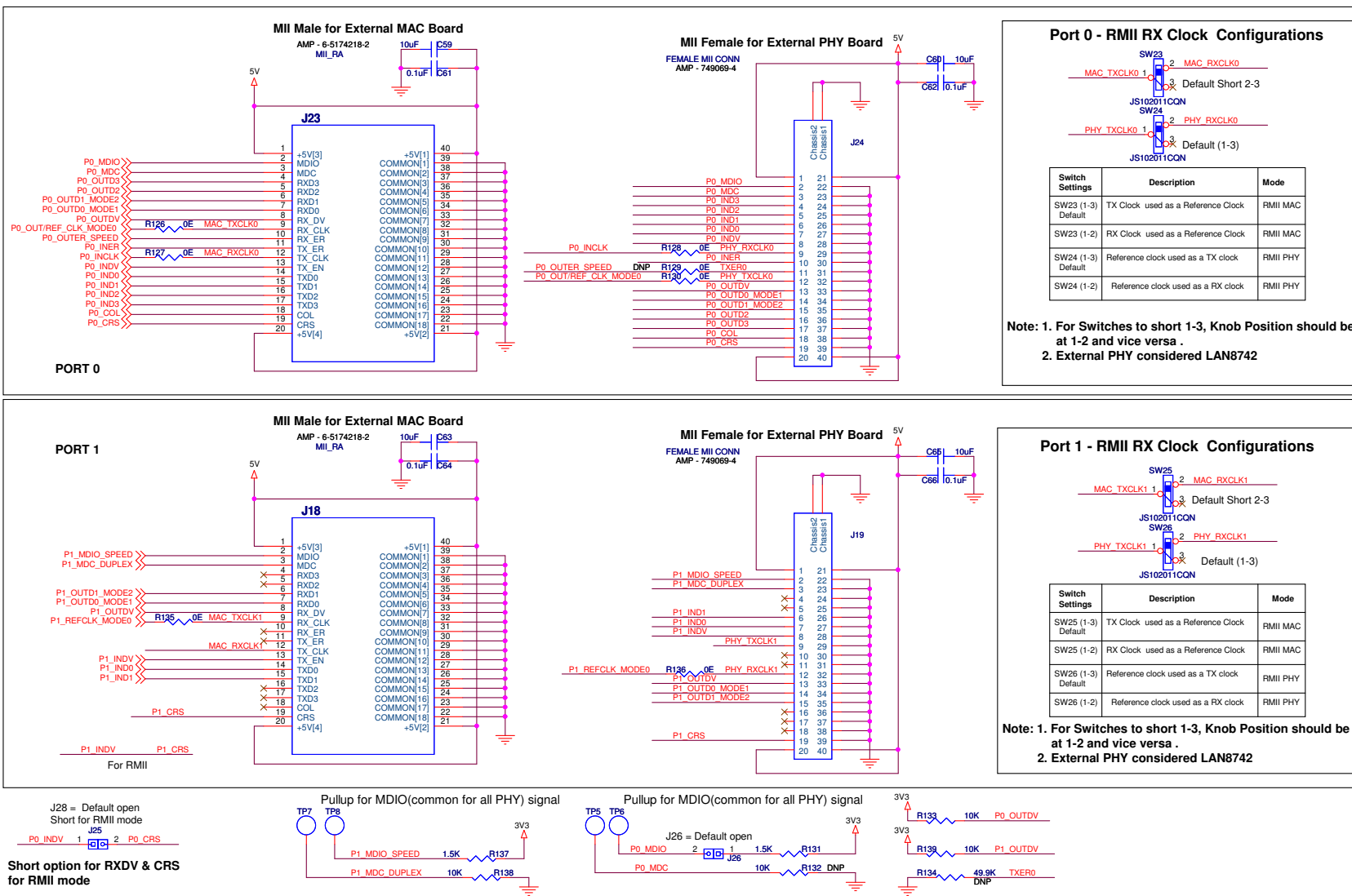
FIGURE B-9: EVB-LAN9353 EVALUATION BOARD SCHEMATIC 9
