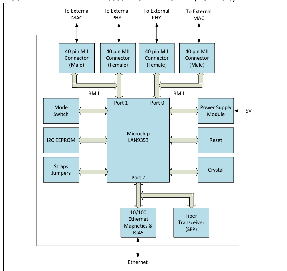
FIGURE 1-1: EVB-LAN9353 BLOCK DIAGRAM (CONFIG 9)
