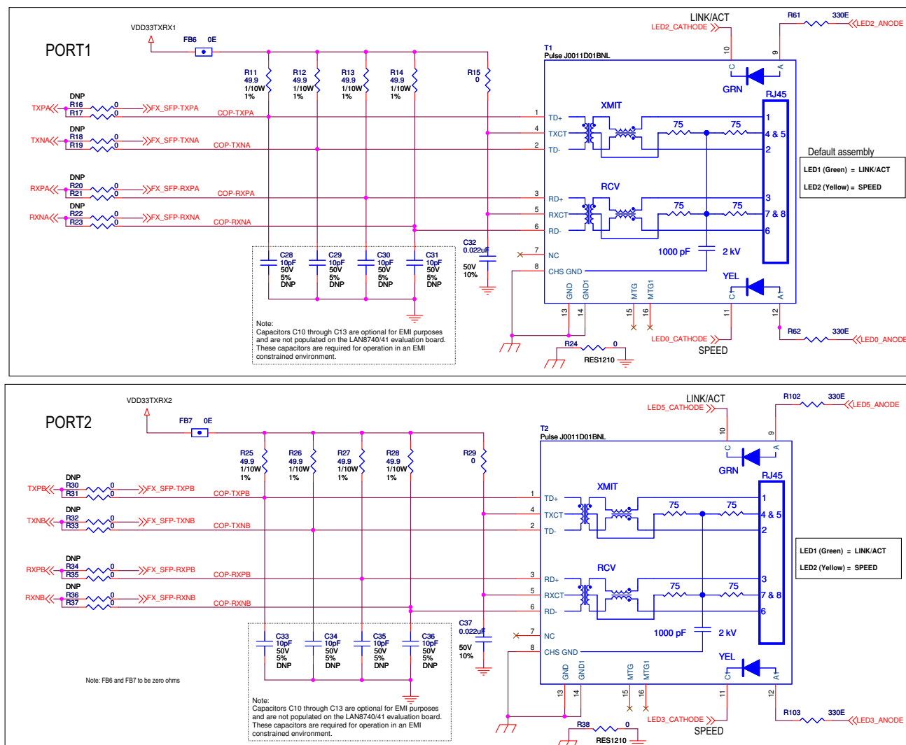
FIGURE B-4: EVB-LAN9353 EVALUATION BOARD SCHEMATIC 4
