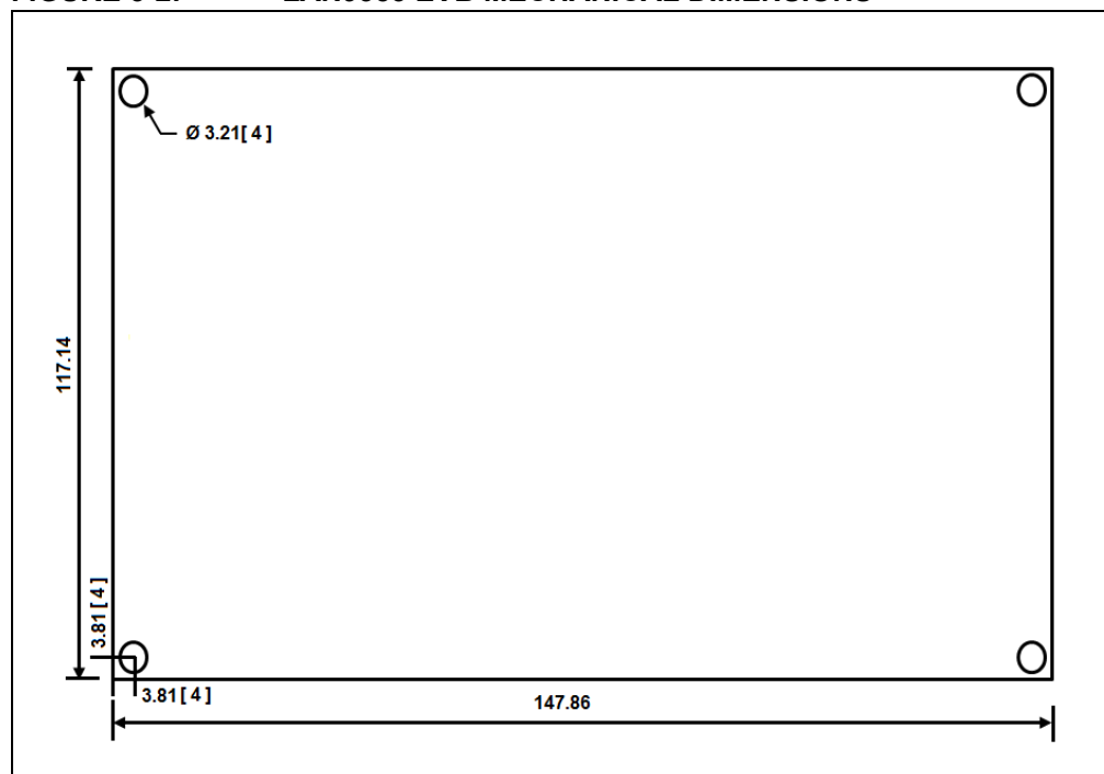
FIGURE 3-2: LAN9353 EVB MECHANICAL DIMENSIONS
