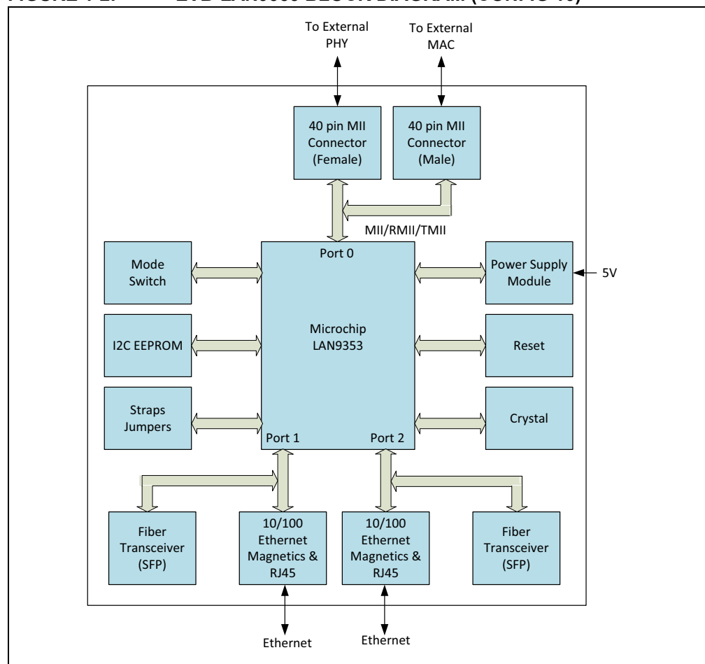
FIGURE 1-2: EVB-LAN9353 BLOCK DIAGRAM (CONFIG 10)
