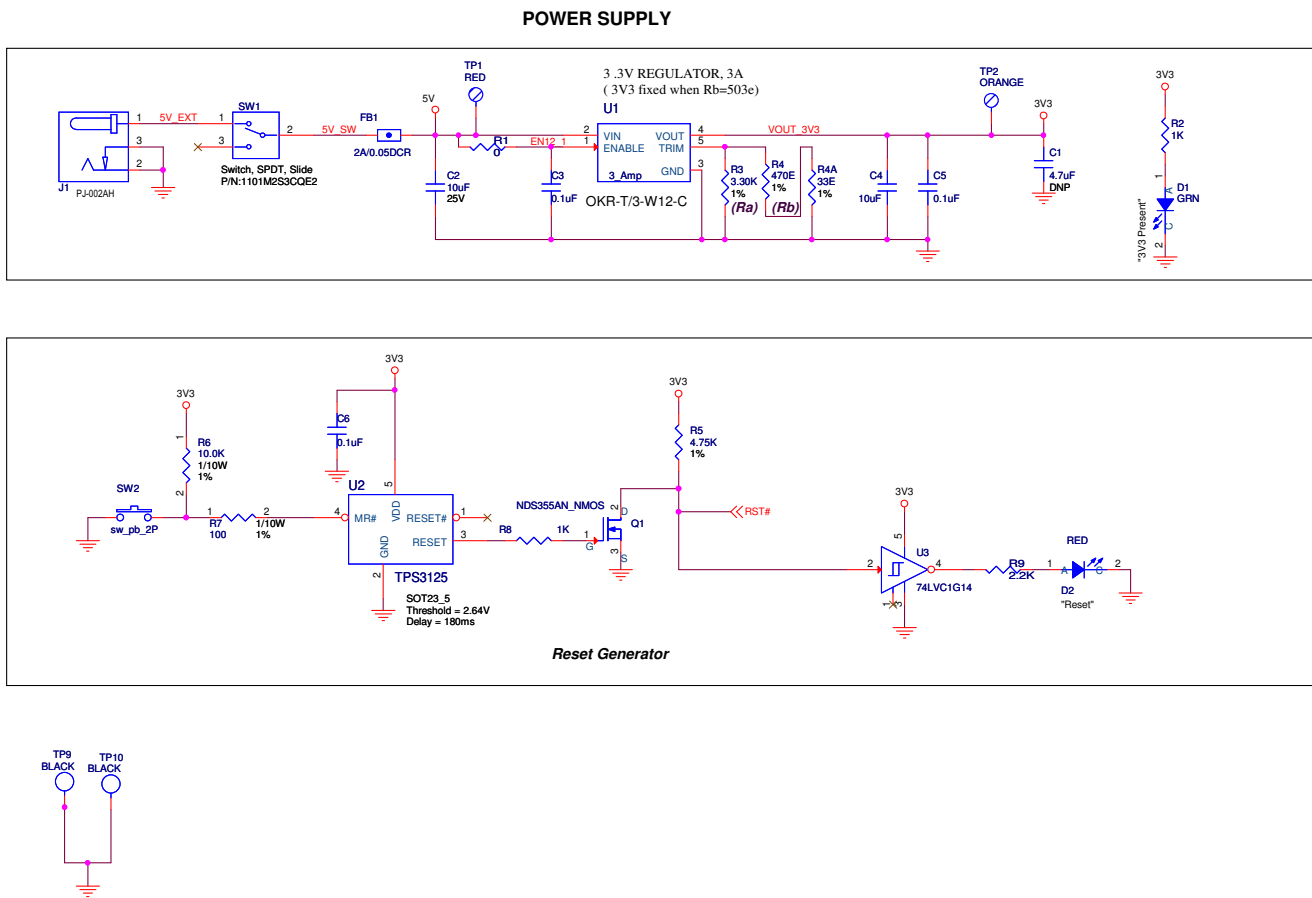
FIGURE B-2: EVB-LAN9353 EVALUATION BOARD SCHEMATIC 2
