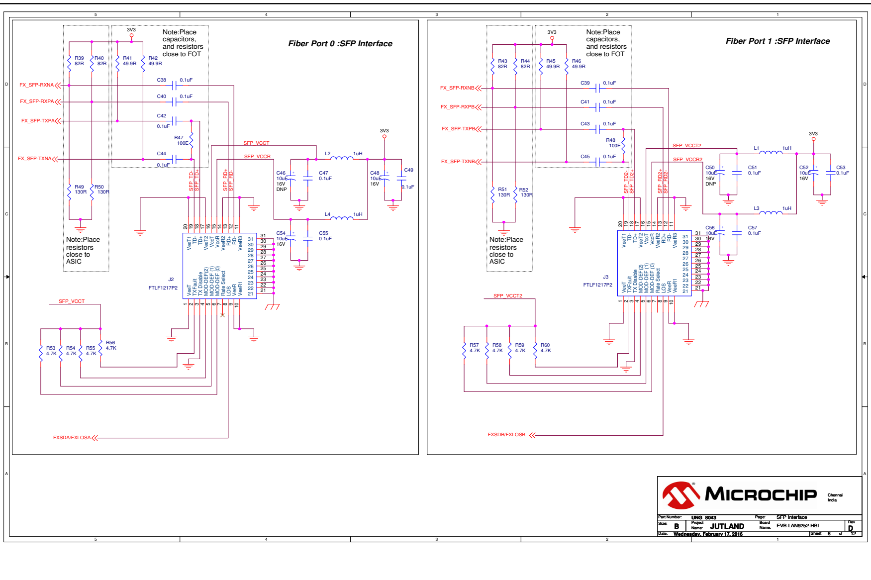
FIGURE B-4: EVB-LAN9252-HBI+ SCHEMATIC SFP INTERFACE
