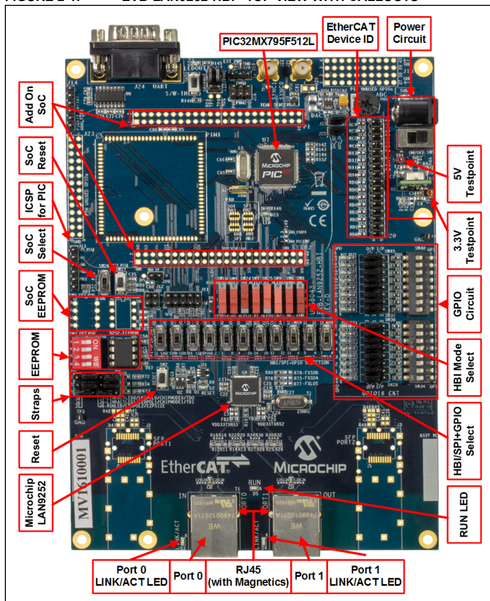
FIGURE 2-1: EVB-LAN9252-HBI+ TOP VIEW WITH CALLOUTS
