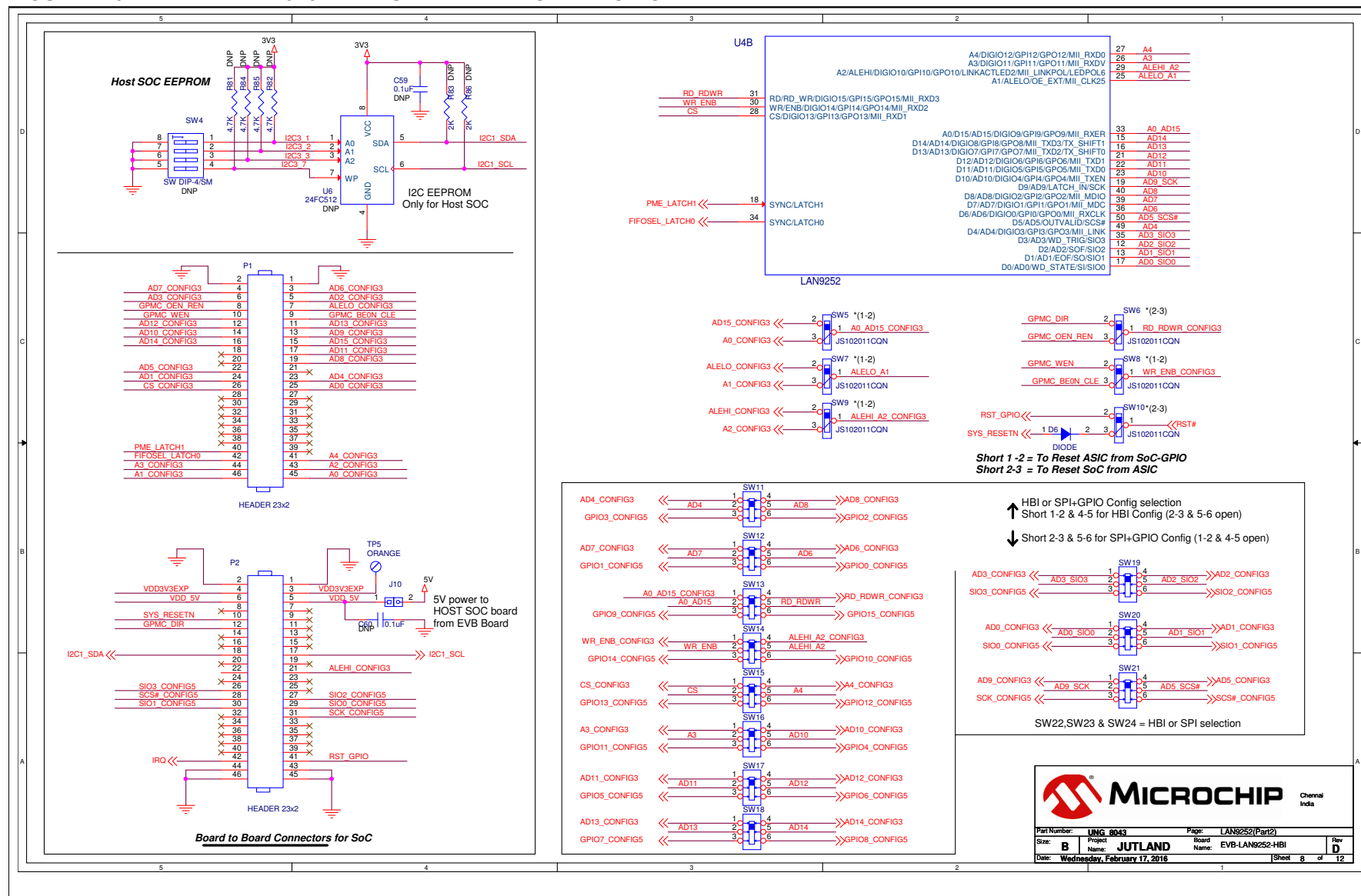
FIGURE B-6: EVB-LAN9252-HBI+ SCHEMATIC BOARD TO BOARD INTERFACE
