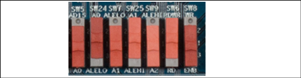
FIGURE 2-5: MULTIPLEXED HBI MODE SELECTION
