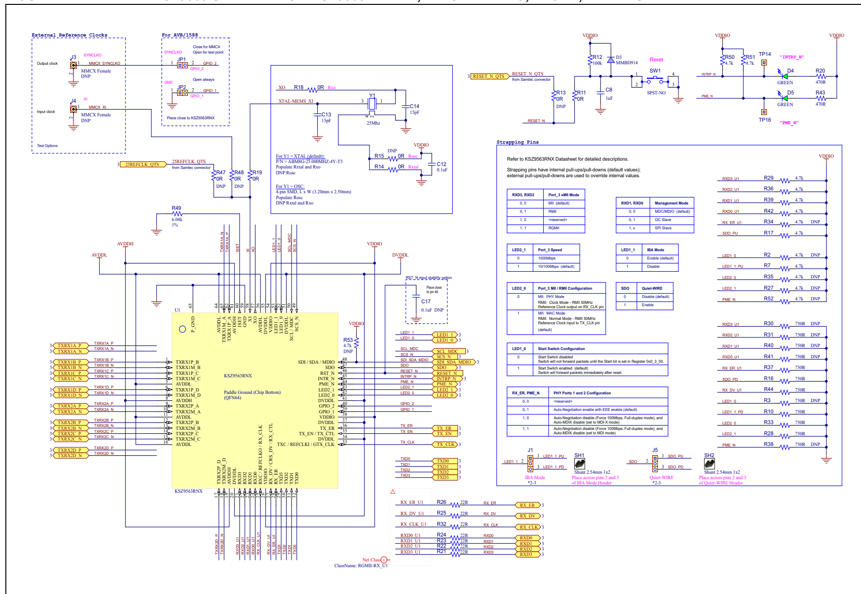
FIGURE B-1: EVB-KS29563 SCHEMATICS – KS29563 DEVICE, PIN STRAPPING, CLOCK, AND RESET
