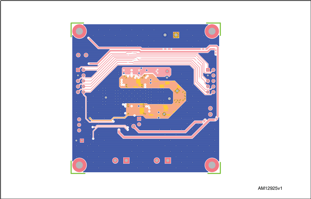
Figure 5. EVAL6470PD - layout (inner layer 3)
