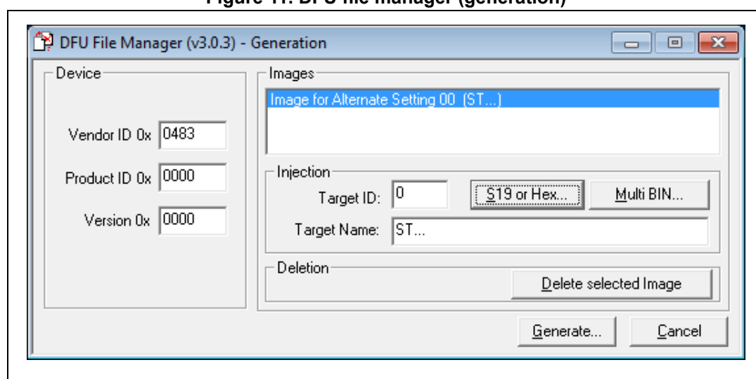
Figure 11. DFU file manager (generation)
