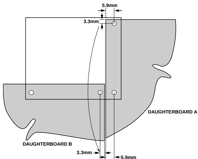
Figure 4. Maximum Board Dimensions for Connector Placement
