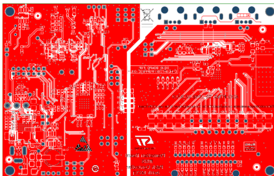
Figure 8. Assembly BOTTOM
