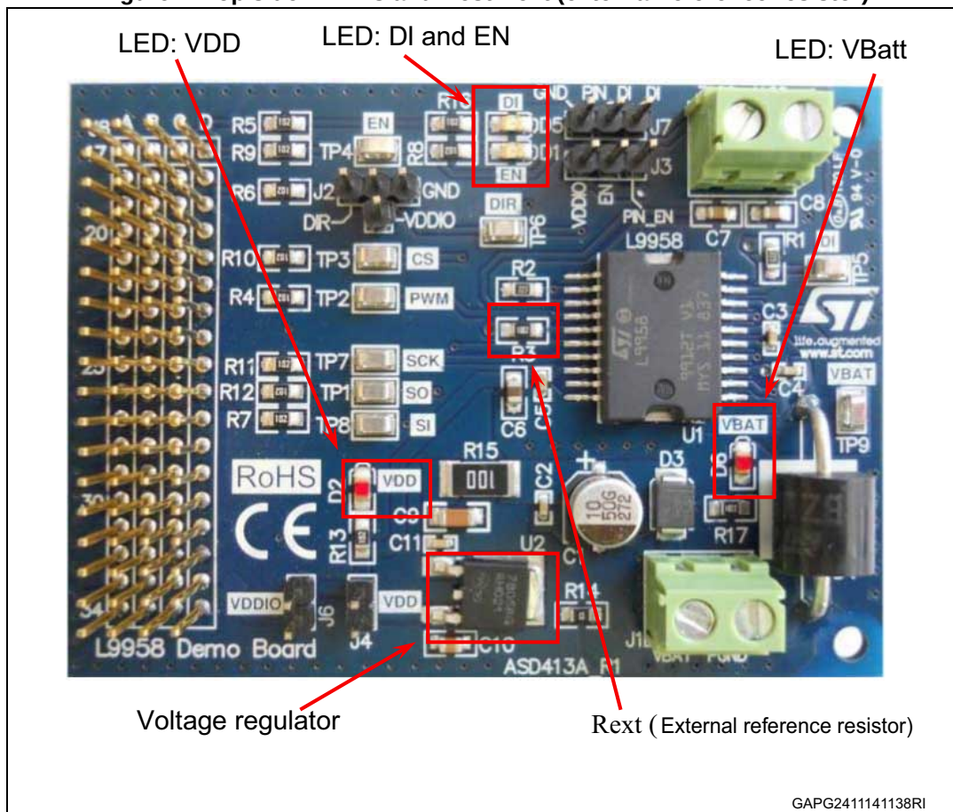
Figure 2. Top side – LEDs and Rest Rext (external reference resistor)
