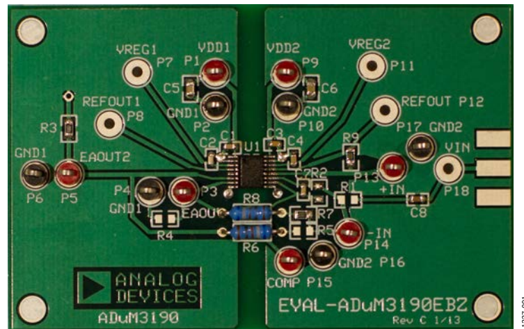
Figure 1. EVAL-ADuM3190EBZ
