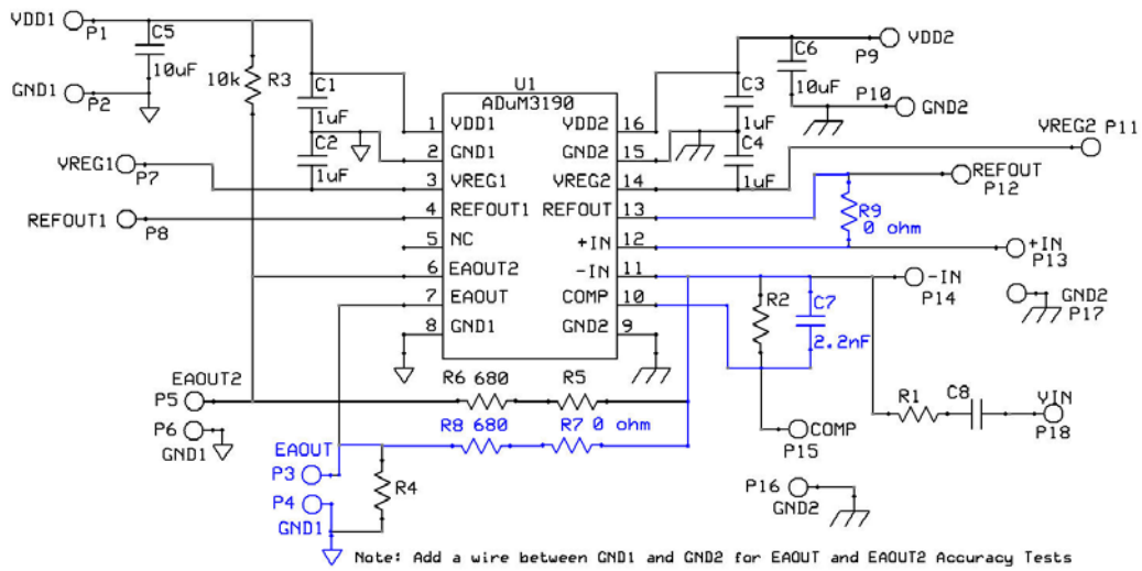
Figure 2. EVAL-ADuM3190EBZ Schematic
