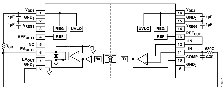
Figure 4. ADuM3190 Test Circuit 2
