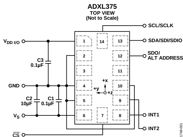
Figure 2. Schematic
