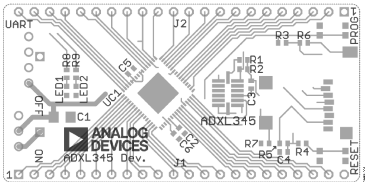
Figure 6. ADXL345 Development Board Layout
