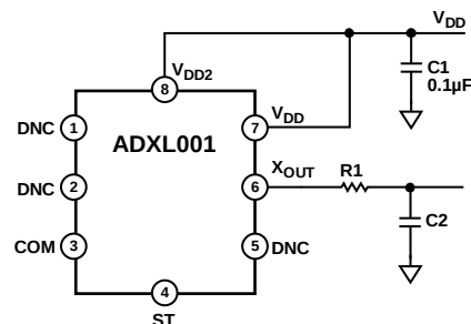
Figure 1. EVAL-ADXL001 Schematic
