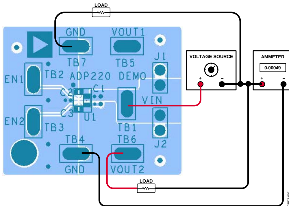
Figure 7. Ground Current Measurement
