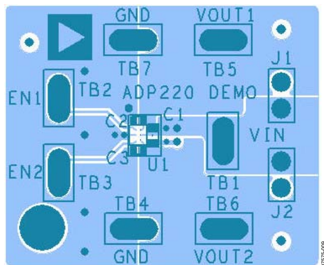
Figure 9. Typical Board Layout, Top Side
