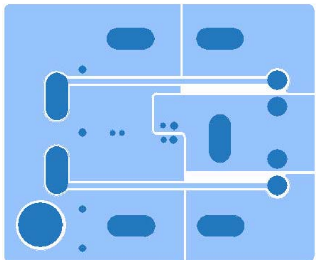
Figure 10. Typical Board Layout, Bottom Side
