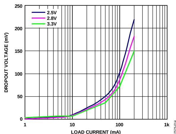
Figure 6. Dropout Voltage vs. Load Current, V_{OUT} = 2.8\text{ V}
