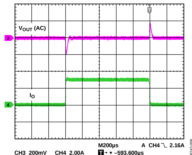
Figure 6. Load Dynamic Without C_{FF}
