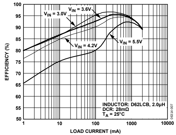
Figure 6. Efficiency—ADP2107-EVAL (2.5 V Output)
