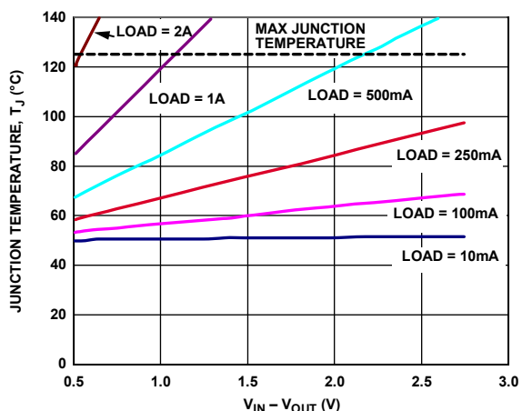
Figure 15. 500 mm² of PCB Copper, T_A = 50^\circ\text{C} , LFCSP
