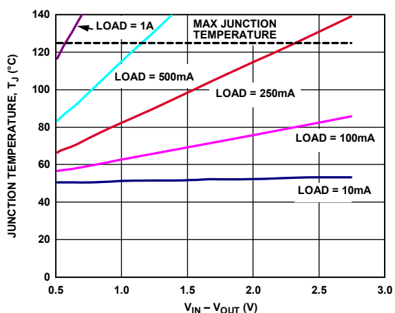
Figure 16. 0 mm² of PCB Copper, T_A = 50^\circ\text{C} , LFCSP
