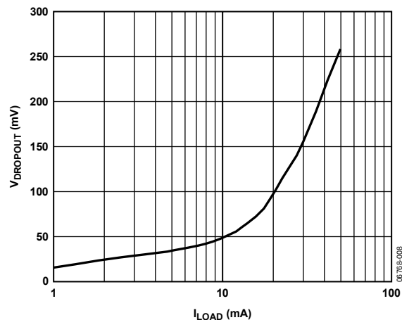
Figure 8. Dropout Voltage vs. Load Current
