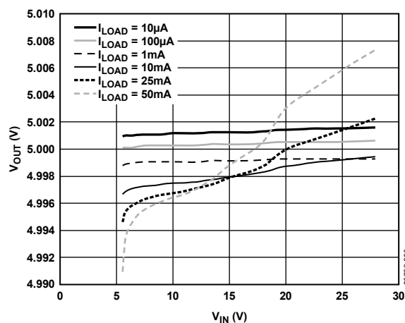
Figure 6. ADP1720 Line Regulation
