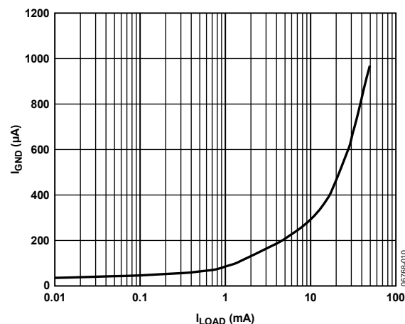
Figure 10. Ground Current vs. Load Current
