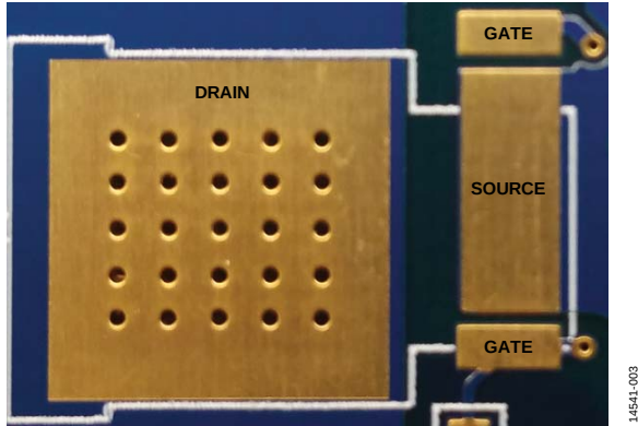
Figure 3. Multipackage N-Channel MOSFET Footprint
