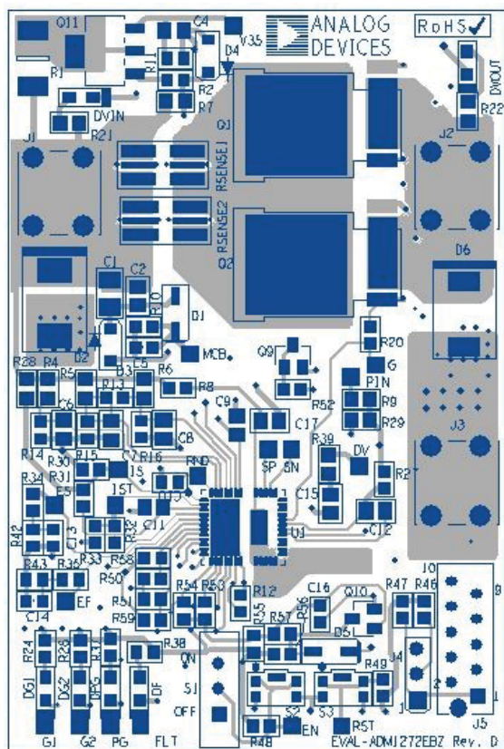
Figure 7. Top Layer 1
