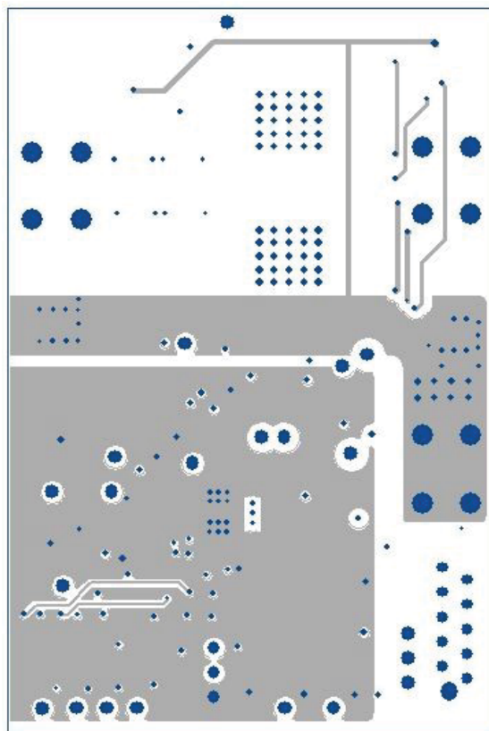
Figure 9. Inner Layer 3
