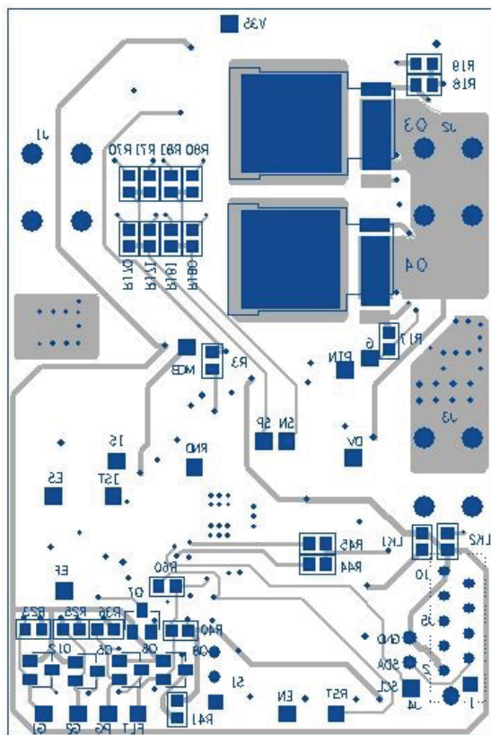
Figure 10. Bottom Layer
