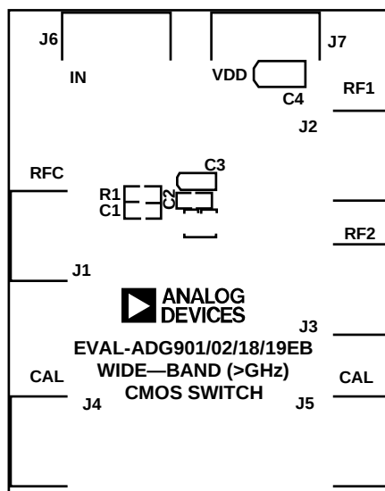
Figure 5. ADG901/ADG902/ADG918/ADG919 Silkscreen
