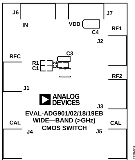
Figure 1. ADG901/ADG902/ADG918/ADG919 Evaluation Board
