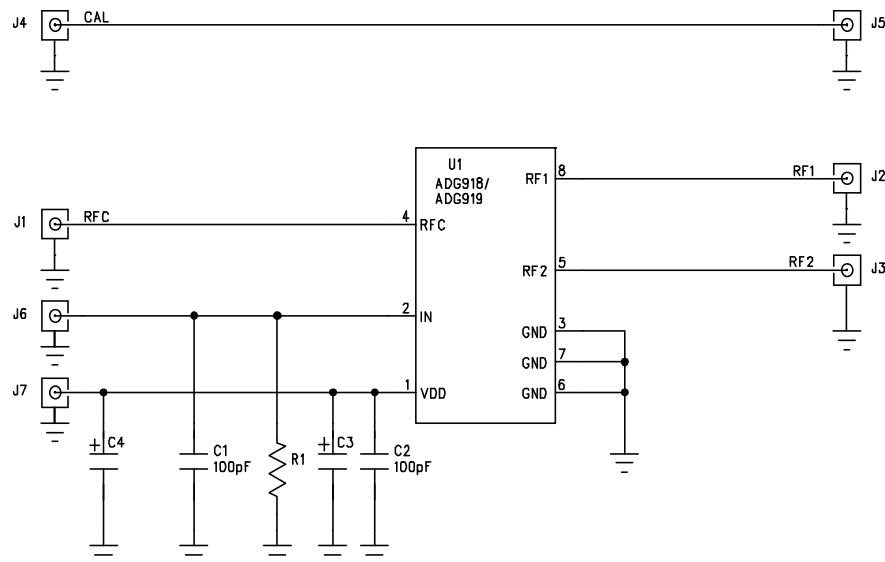
Figure 4. ADG918/ADG919 Schematic
