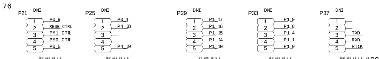
Figure 50. MCU Pin Connections
