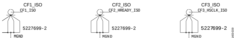
Figure 39. Isolated Connections of CF Pins
