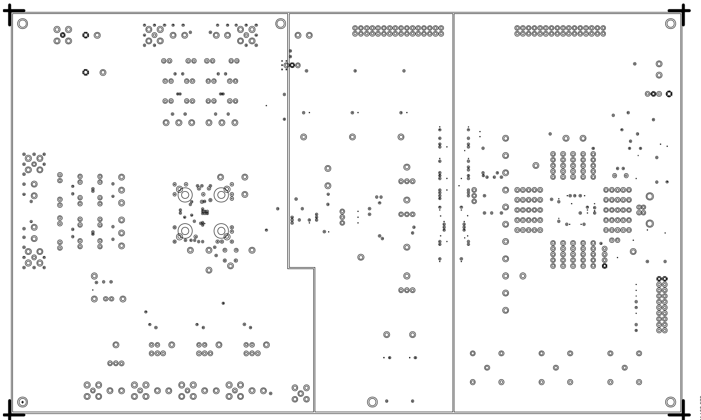
Figure 73. Layer 3
