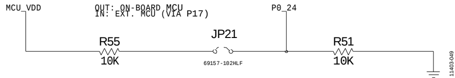
Figure 49. MCU Override
