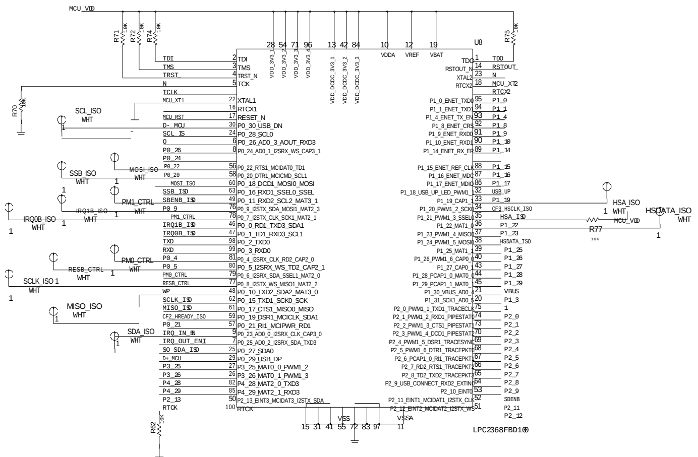
Figure 47. LPC2368 Schematic
