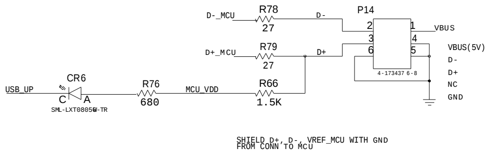
Figure 70. USB Interface
