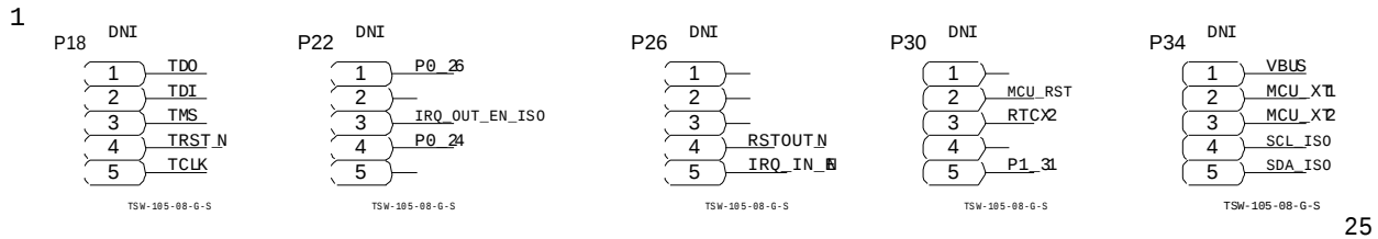
Figure 49. MCU Override
