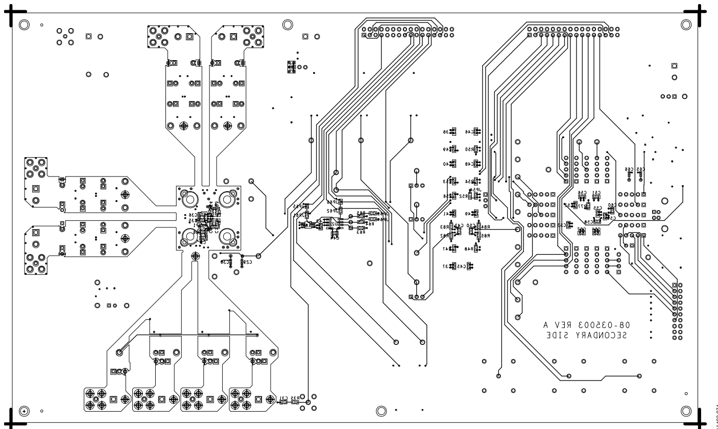
Figure 74. Bottom Layer
