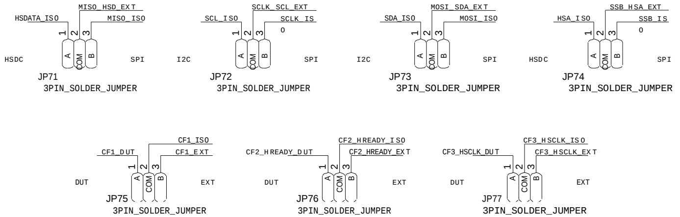
Figure 44. I/O Selection
