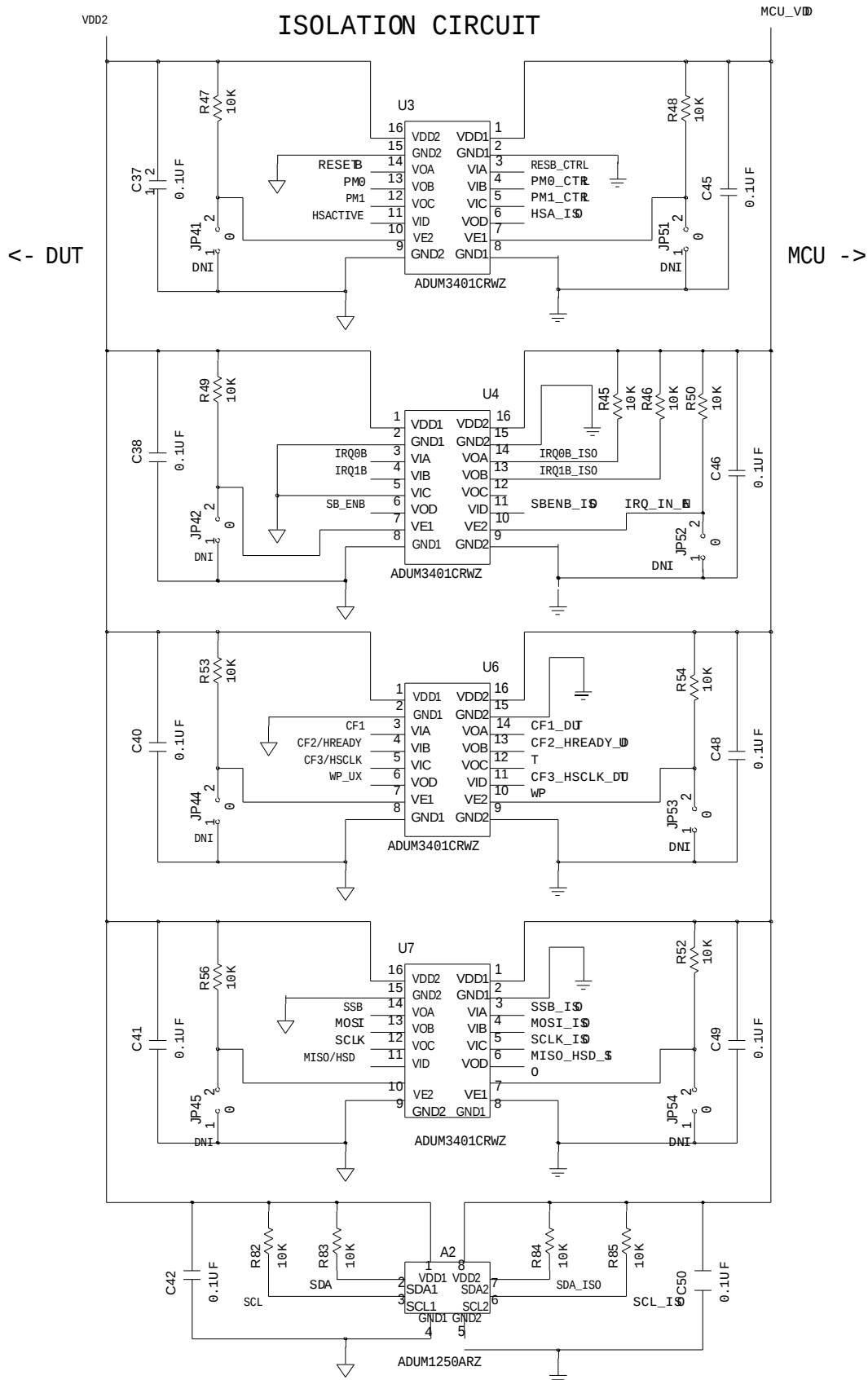
Figure 45. Isolation Circuitry
