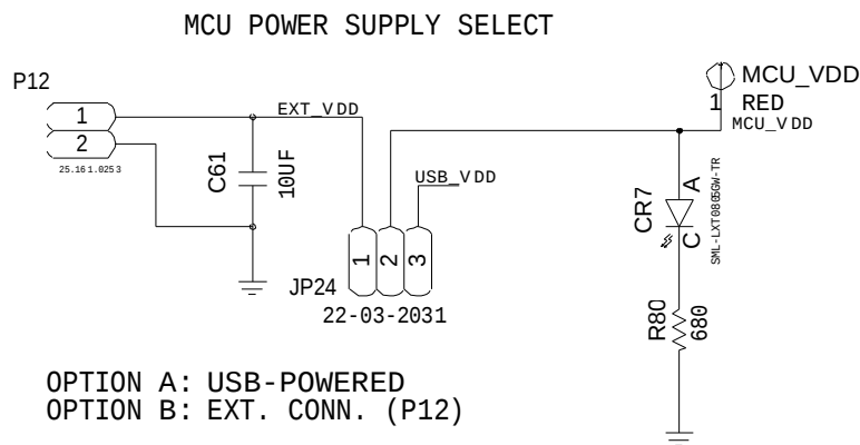
Figure 53. MCU Power Supply Selection
