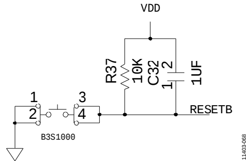
Figure 68. ADE7854A/ADE7858A/ADE7868A/ADE7878A Reset Circuit
