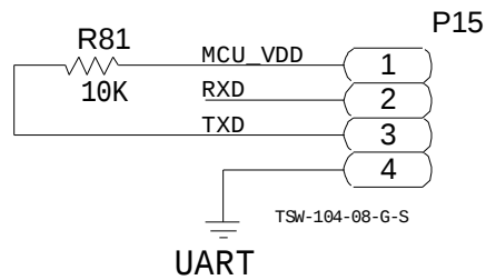
Figure 69. UART Circuit
