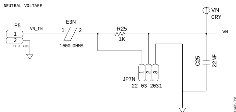
Figure 58. VN Circuit
