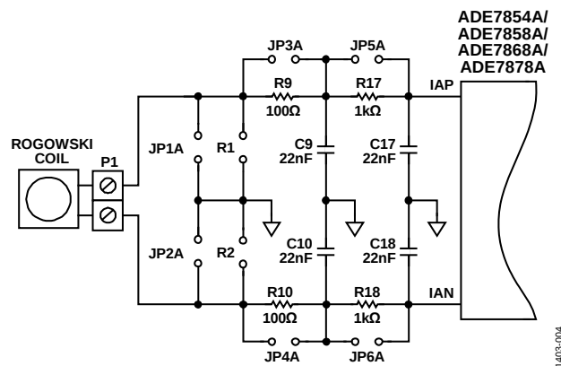
Figure 4. Example of a Rogowski Coil Connection
