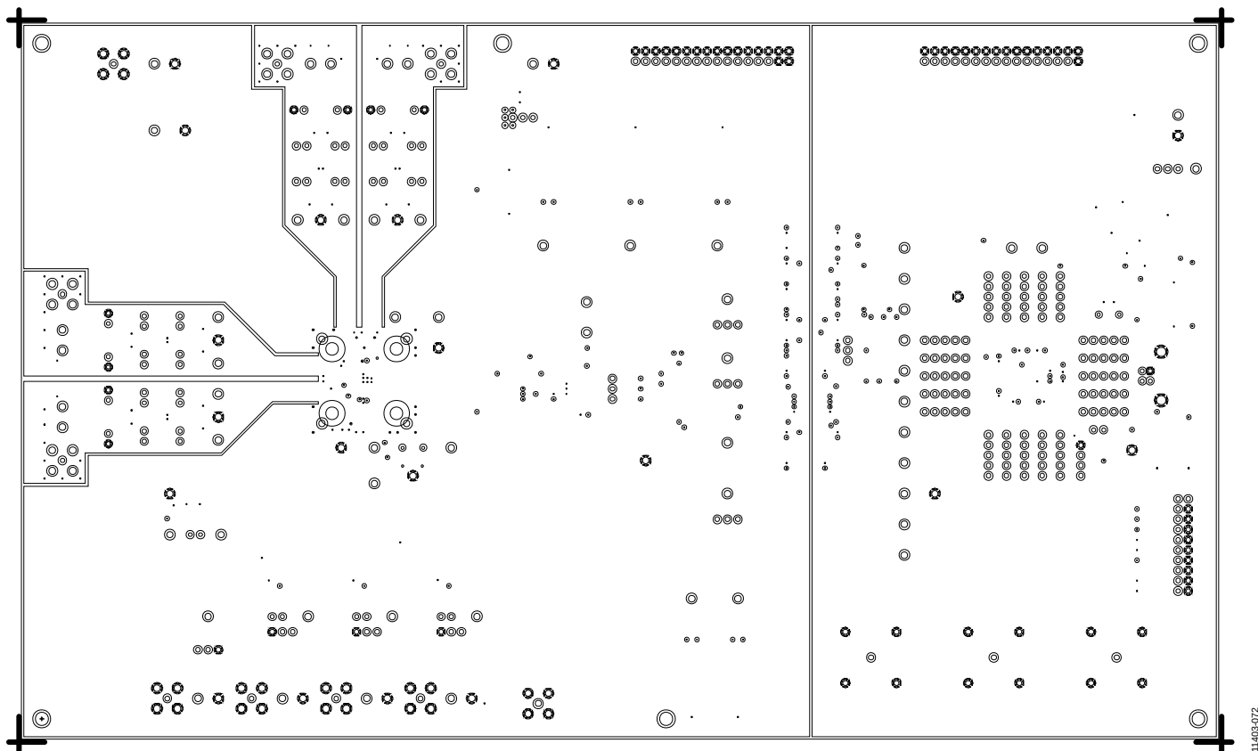
Figure 72. Layer 2
