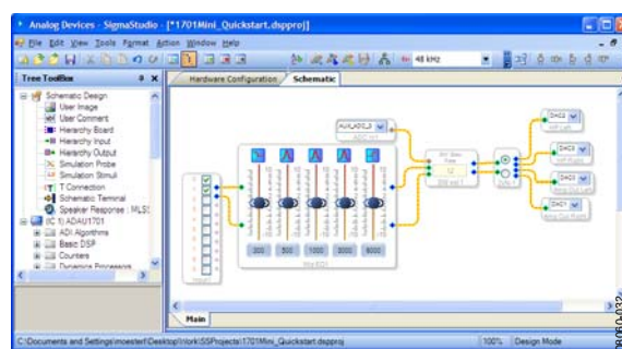
Figure 4. Schematic Tab, Full Design
