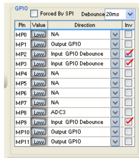
Figure 13. SigmaStudio Multipurpose Pin Configuration for the EVAL-ADAU1701MINIZ
