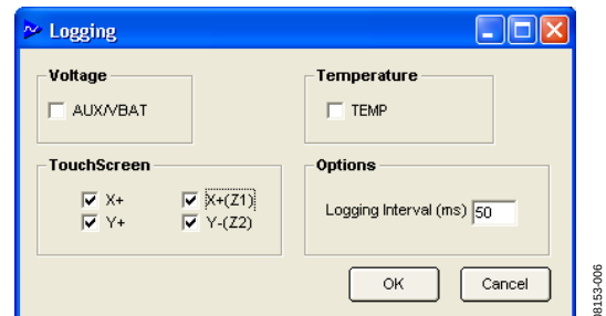
Figure 6. Logging Window
