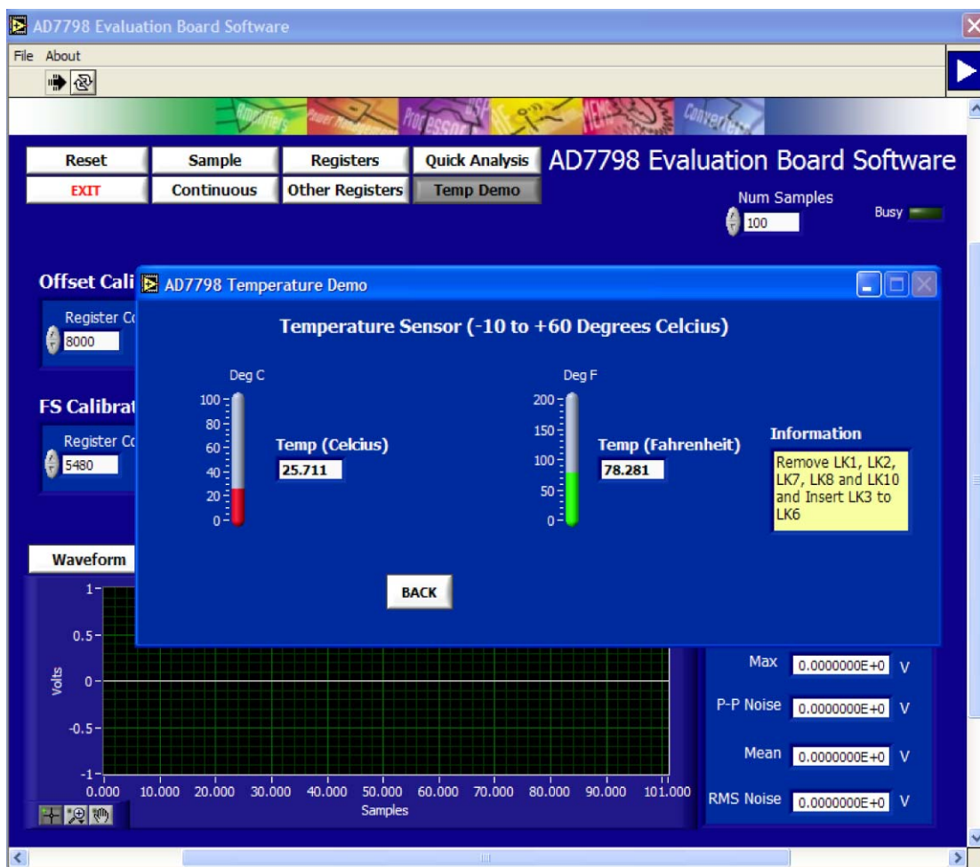
Figure 6. AD7798 Evaluation Software Temperature Demo Window
