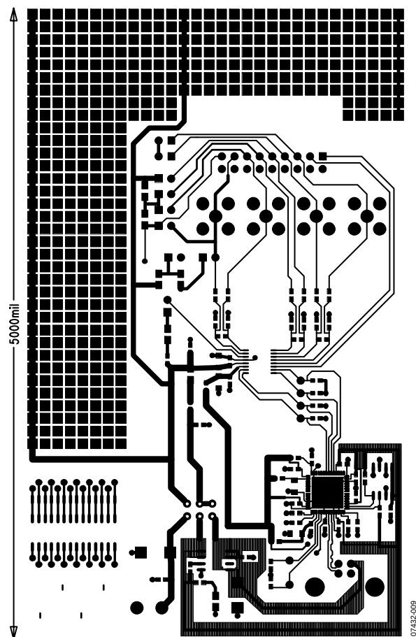
Figure 9. AD7798 Evaluation Board—Component Side Artwork
