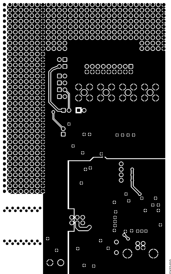
Figure 10. AD7798 Evaluation Board—Solder Side Artwork
