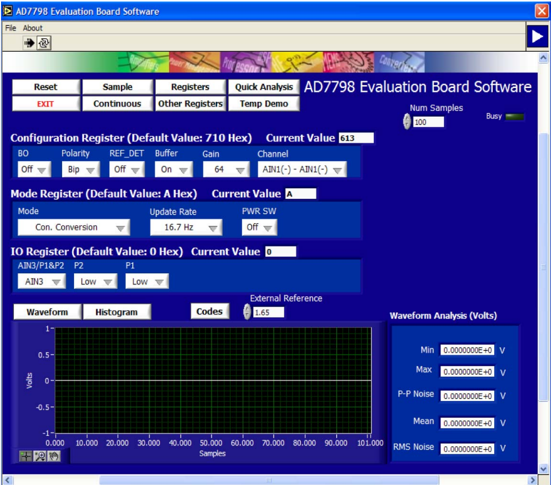
Figure 4. AD7798 Evaluation Software Registers Window
