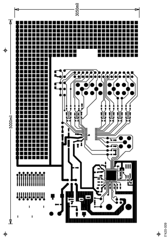
Figure 8. AD7795 Evaluation Board Component Side Artwork
