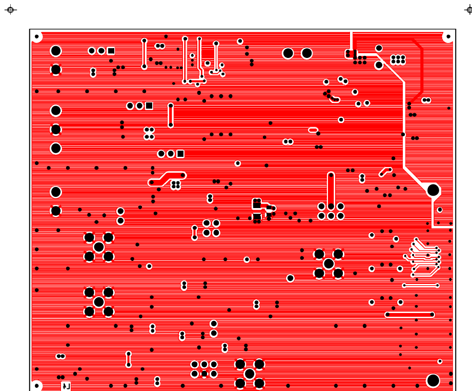
Eval-AD7492SDZ (Rev. A) Top Side View. Bottom Side Layer 4
