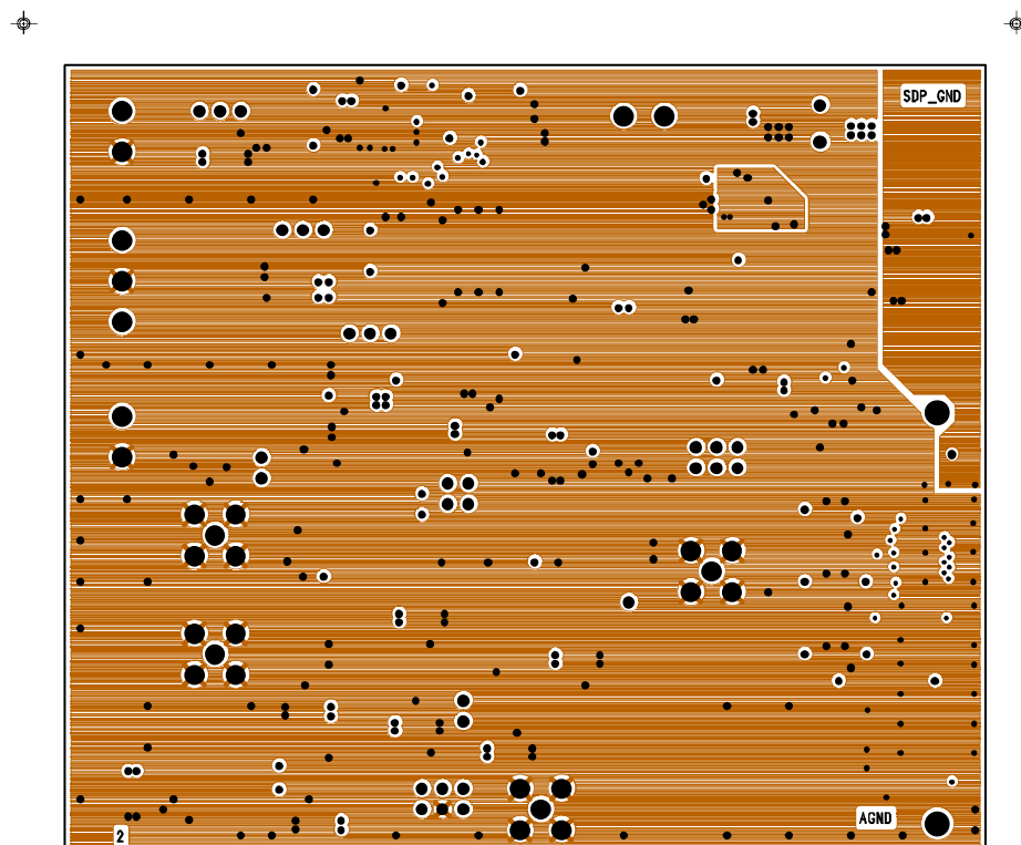
Eval-AD7492SDZ (Rev. A) Top Side View. Layer 2 – Ground
