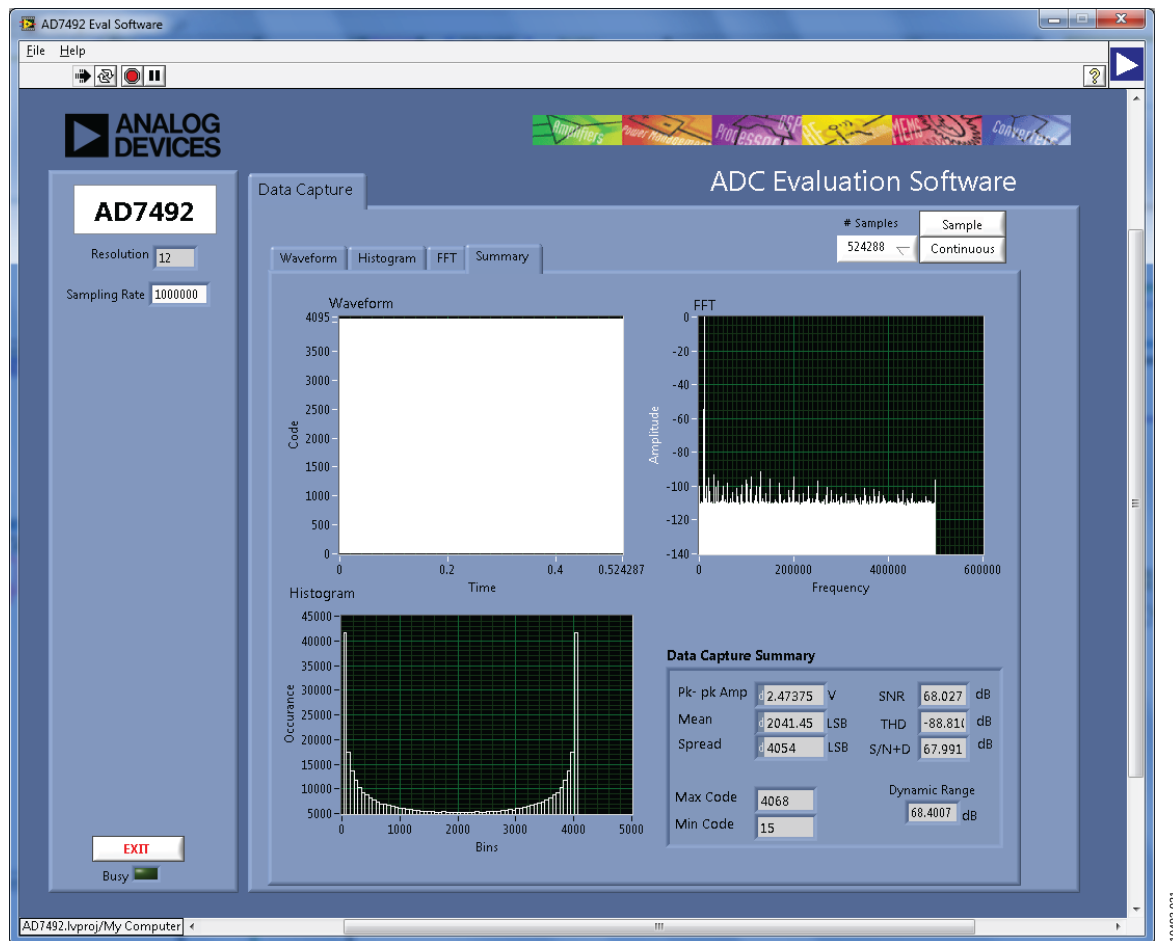
Figure 20. Data Capture/Summary Tab
