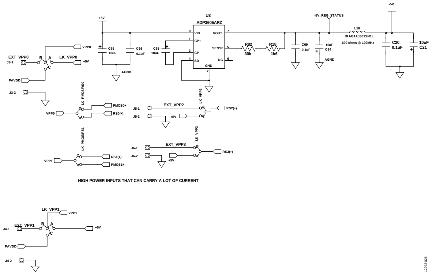
Figure 28. EVAL-AD7293SDZ Schematic, VPP and Negative Power Supply Block
