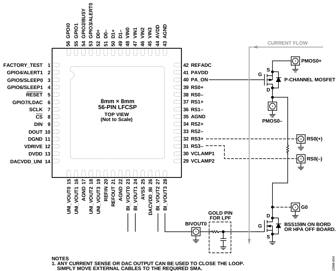
Figure 4. EVAL-AD7293SDZ Loop Configuration
