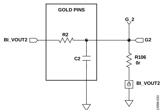
Figure 35. EVAL-AD7293SDZ Schematic, BI_VOUT2 Filter Block
