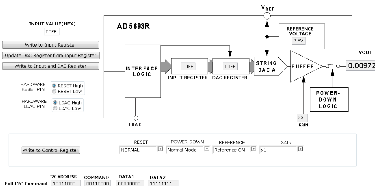
Figure 5. AD5693R Evaluation Board Main Window
