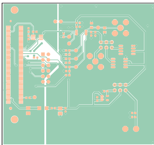
Figure 9. Component Side PCB Drawing
