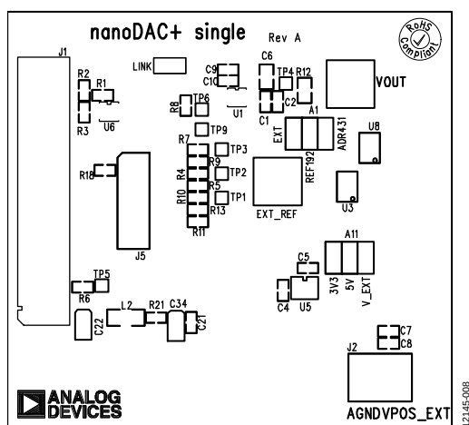
Figure 8. Component Placement Drawing
