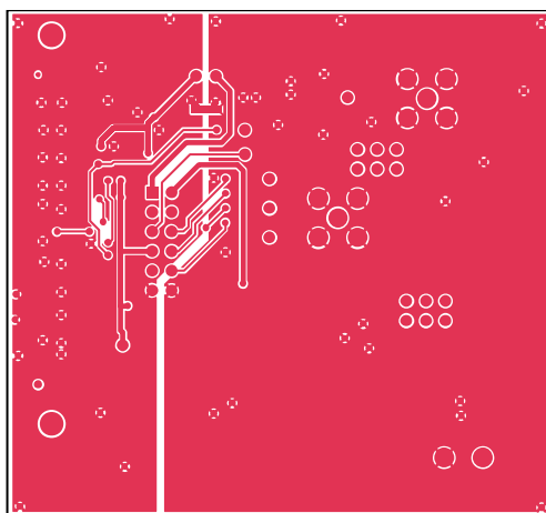
Figure 10. Solder Side PCB Drawing
