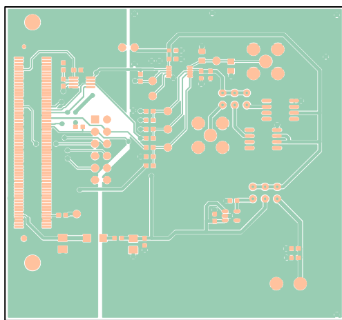
Figure 9. Component Side PCB Drawing
