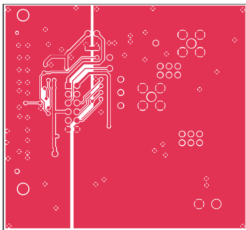
Figure 10. Solder Side PCB Drawing
