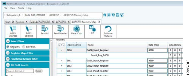
Figure 5. AD5675R Memory Map
