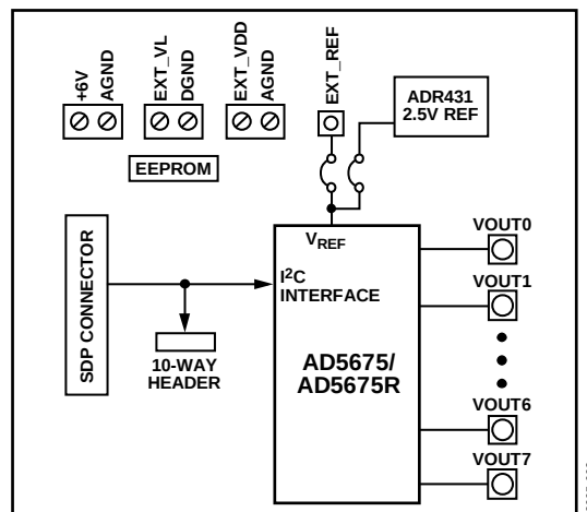
Figure 7. Evaluation Board Block Diagram
