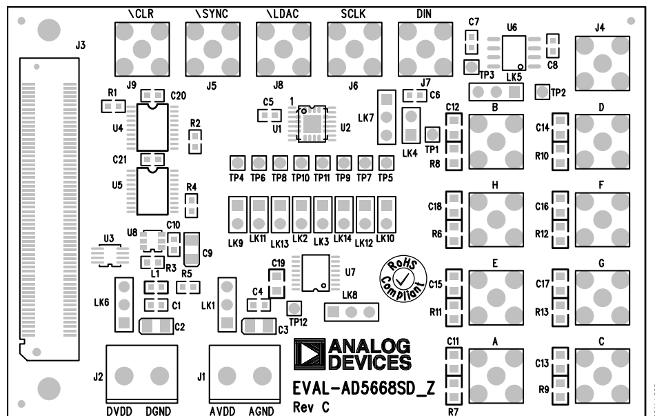
Figure 7. Component Placement Drawing
