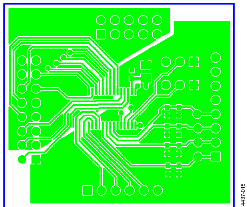
Figure 15. EVAL-AD5344DBZ Daughter Board Top Side Routing
