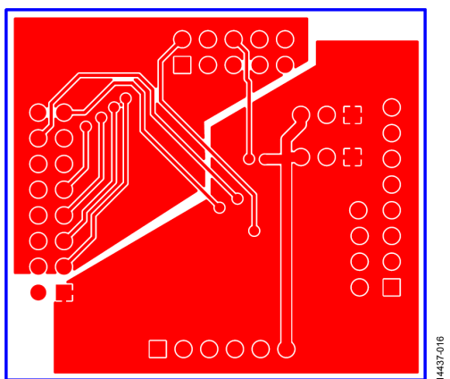
Figure 16. EVAL-AD5344DBZ Daughter Board Bottom Side Routing
