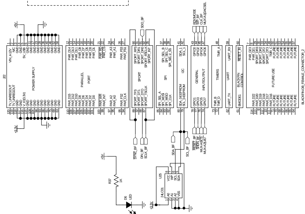
Figure 14. Schematic of SDP-B Connector
